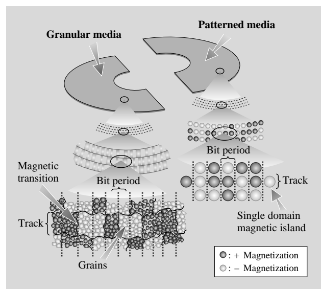
Fig. 5—Outline of Patterned Media Technology. Patterned media replaces the many random, small grains of continuous film, granular media with one larger magnetic island that acts to store a single bit. By making the islands larger than the individual grains, the magnetic bits can be scaled to smaller size (i.e. higher density) and remain thermally stable.
