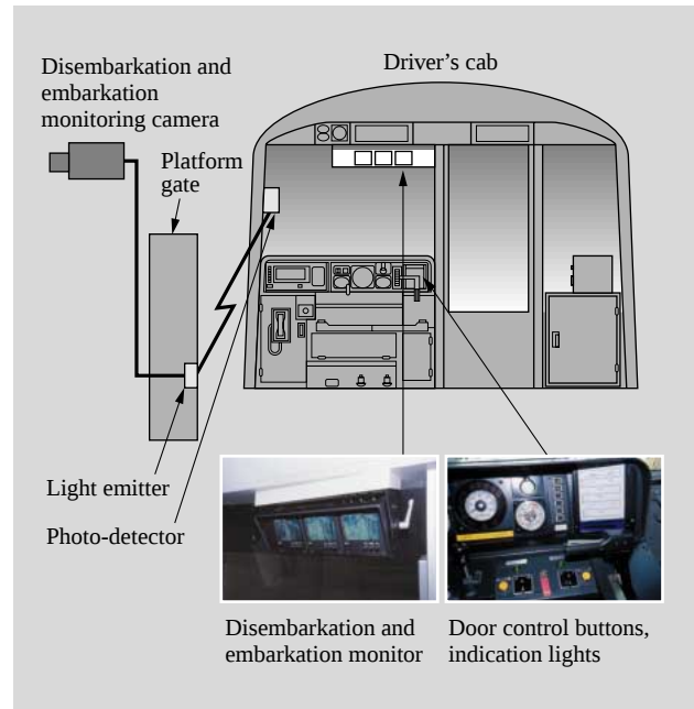
Fig. 3—Monorail Control Platform. It supports one-person operations, and is more convenient for train operator.
