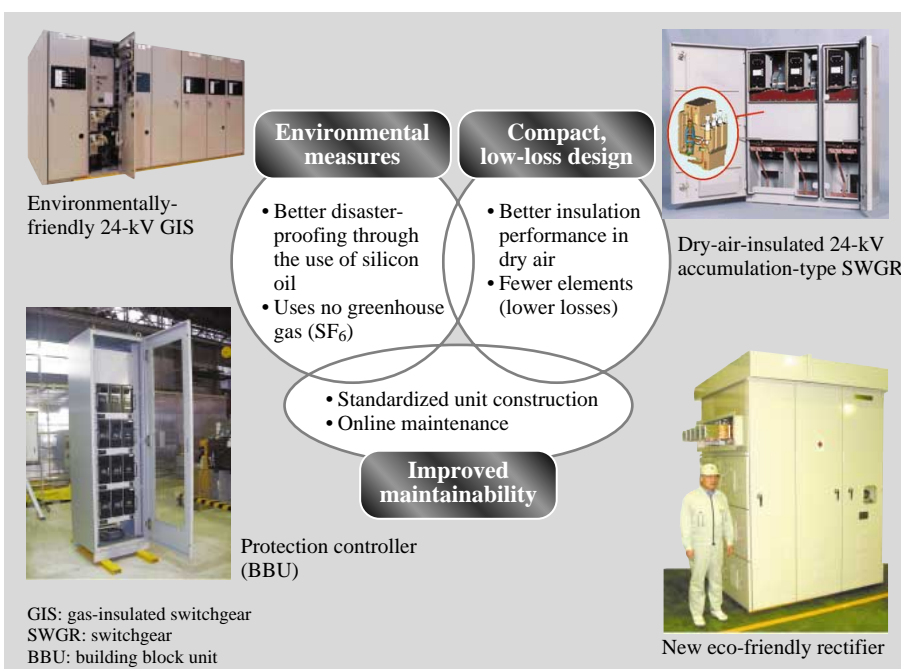
Fig. 1—Environmental Railway Substation System.
