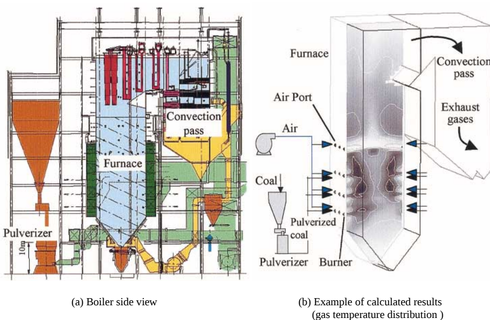
Fig. 1— Combustion Analysis for a Pulverized-Coal-fired Boiler. A means of predicting the state of combustion is indispensable in the design of a furnace, which is the heart of the boiler. This analysis program calculates the combustion state from the amount of fuel entering from the burners and the amount of air entering from the air ports.
