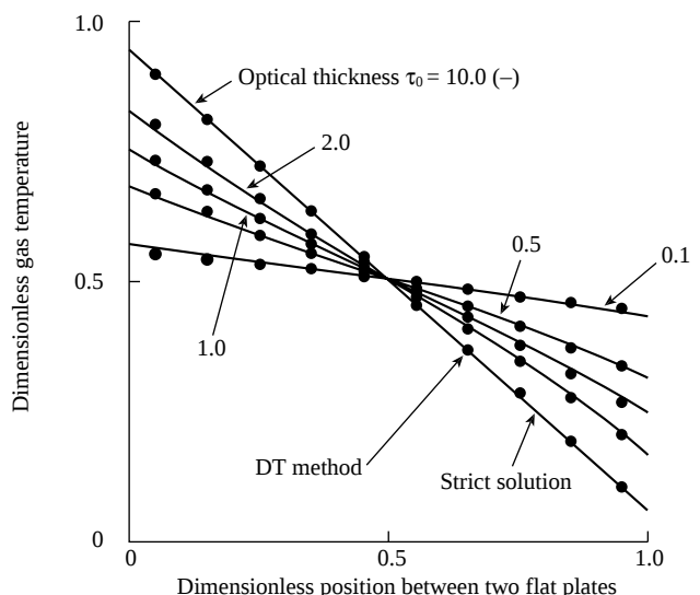
Fig. 3— Comparison of Strict Radiative Transport Solutions and Results of the DT Method.
