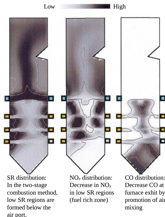
Fig. 2— Examples of Combustion Analysis Within the Furnace. In the two-stage combustion method, the SR near the burner is precisely controlled so as to control the generation and release of gases that pollute the environment.
