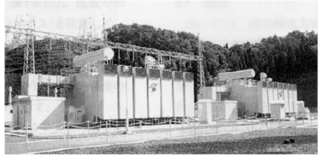
Fig. 4— View of 400-MVA Disassembled-transport Transformer Delivered to the Nanjo Substation of Hokuriku Electric Power Company.
