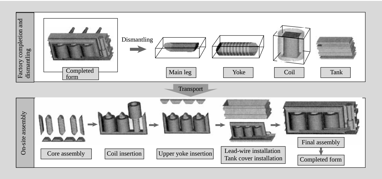
Fig. 1— Work Flow After Factory Completion of a Disassembled-transport Transformer. Main components are dismantled and transported, and then re-assembled at the destination site.
