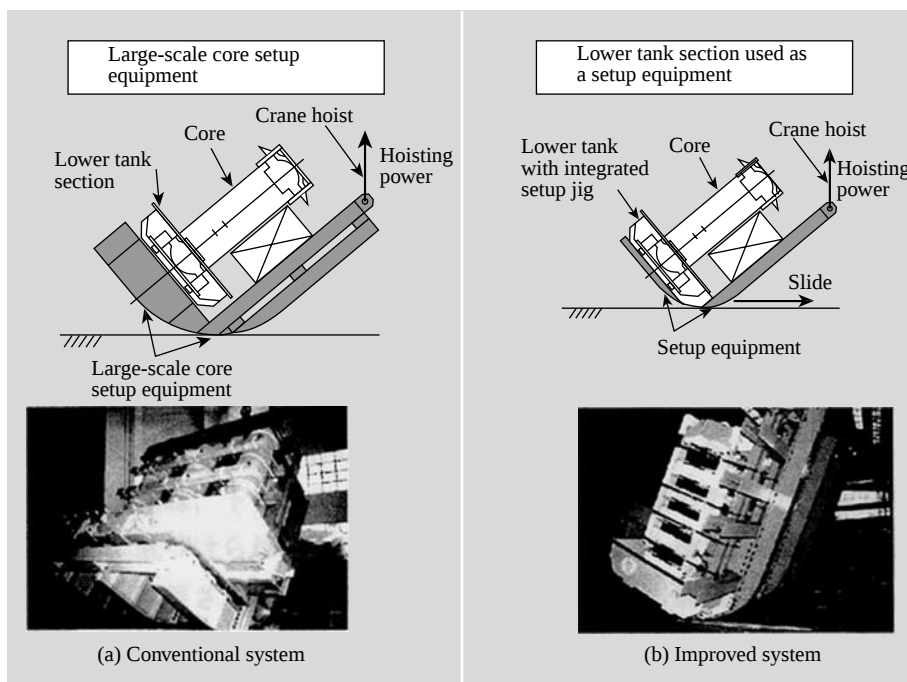
Fig. 2—Improvements in Core Assembly Technology. Operations are simplified by using the lower tank section as a setup equipment.
