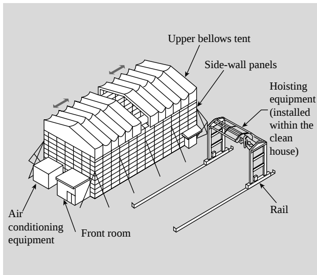
Fig. 3— Clean House Configuration.
