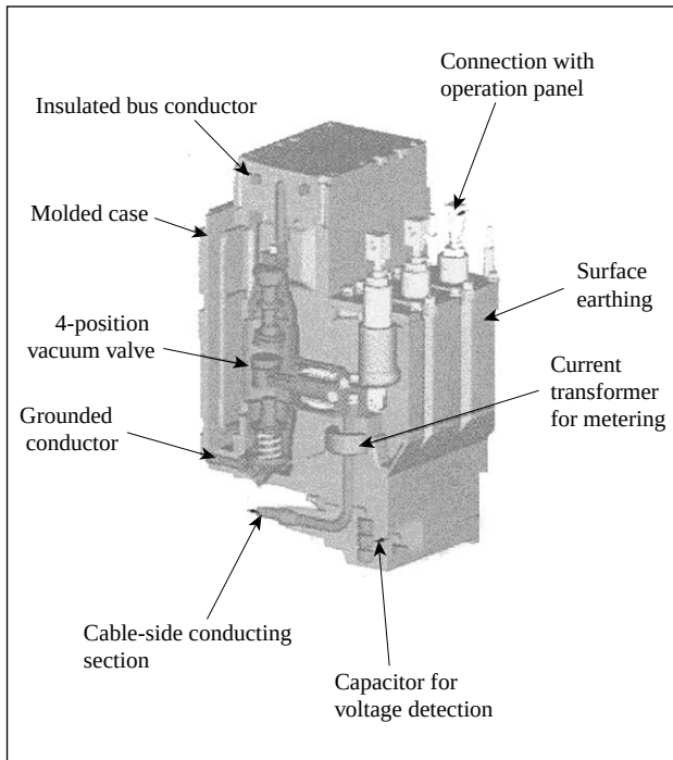
Fig. 3— Cross Section of Main-circuit Section. The entire surface of the epoxy-molded surface is coated with conductive paint and grounded to make maintenance operations safe.
