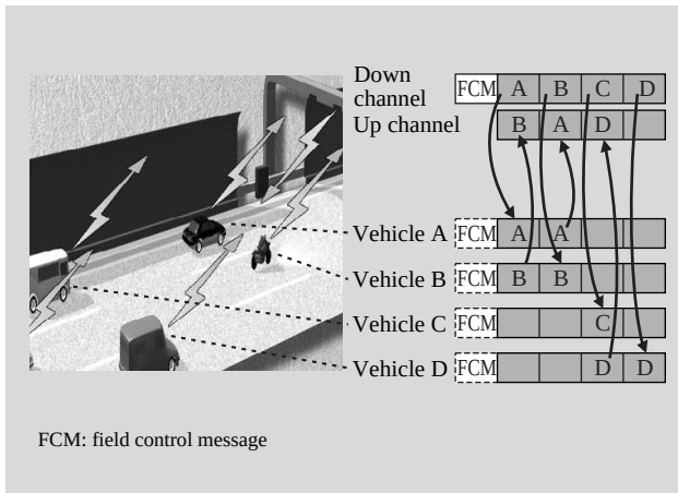
Fig. 6— DSRC Communication Protocol. Assigning one slot to one vehicle makes it possible to communicate with multiple vehicles simultaneously.
