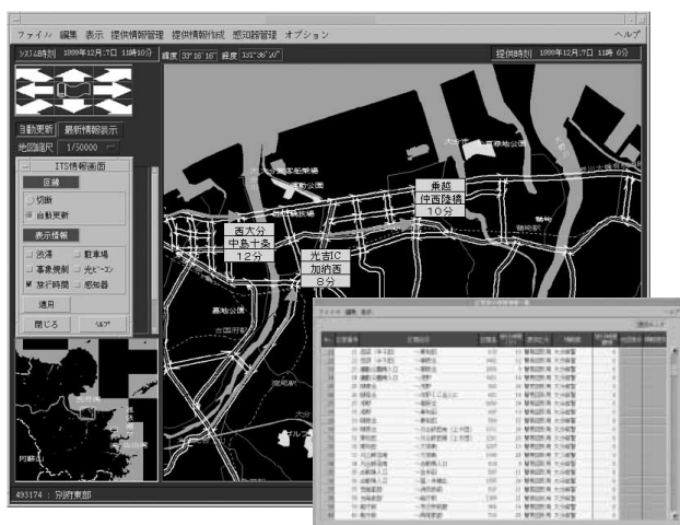
Fig. 4—Example of Control Room Monitor Display. By superimposing section travel times on the digital road map, information provision and management are integrated.
