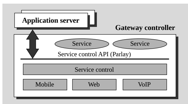
Fig. 3—Service Customization with Open API. The use of an open API in the gateway controller will enable several kinds of network service applications to be provided.
