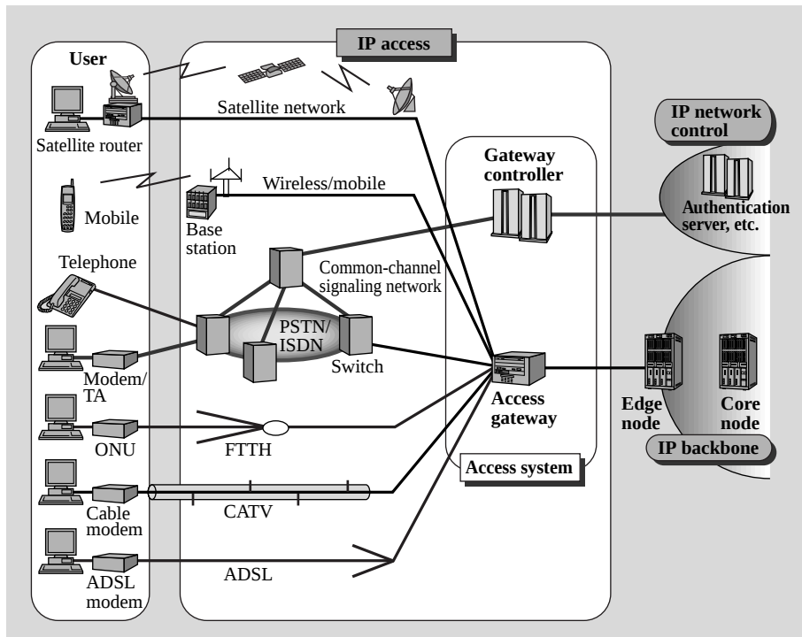
Fig. 2—Hitachi's Concept of Next-generation IP Network and Its Access System.
