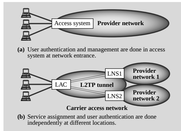
Fig. 1—User Authentication and Management in Access System. In case (b), an L2TP access concentrator (LAC) is placed at the entrance to the carrier network and an L2TP network servers (LNSs) is placed at the entrance to each provider network. L2TP tunneling is used between the LAC and LNSs.
