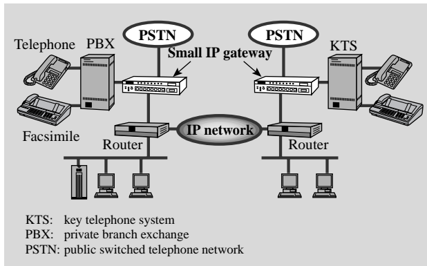
Fig. 3—VoIP Solution for Small Enterprise Networks. This solution integrates existing PBX/key telephone systems with LAN systems by using small IP gateways.
