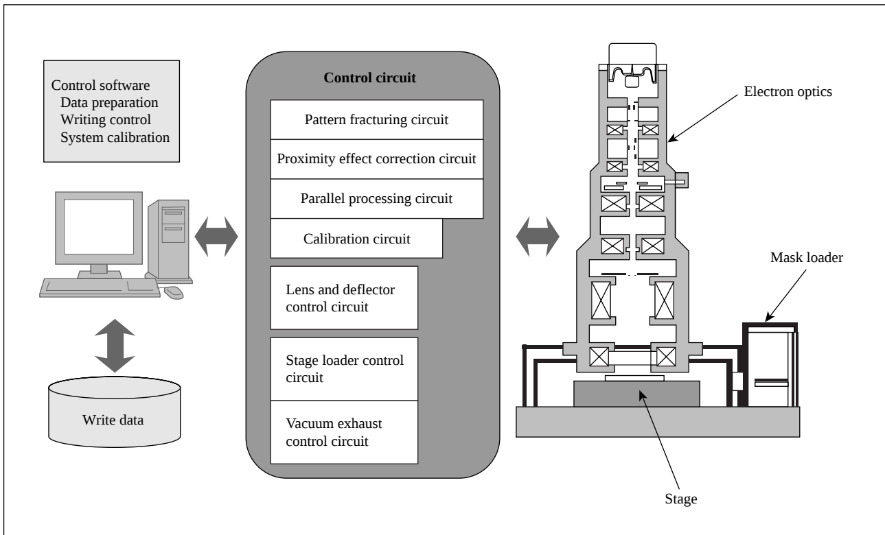
Fig. 3—HL-900M Series System Configuration.
