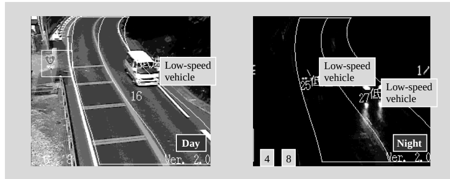
Fig. 8—Example of Image Processing. Day (left) and night (right). Image sensor enables 24-hour monitoring.
