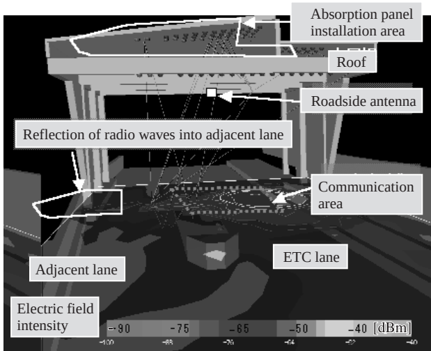
Fig. 6—Example of Propagation Simulation Application. In a study of radio wave conditions at a tollbooth, the optimum installation area for radio frequency absorption panels is calculated using propagation simulation.
