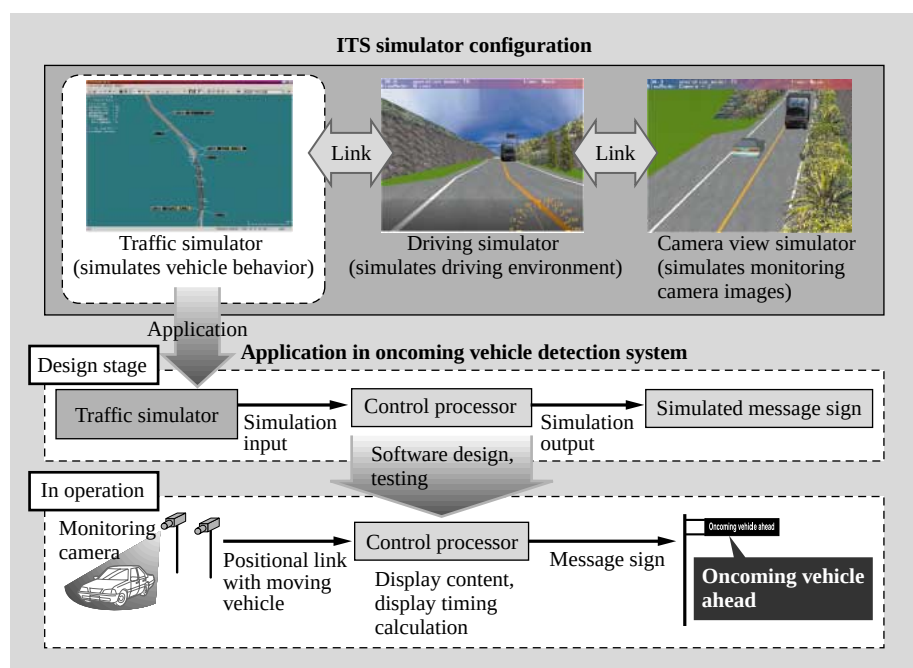
Fig. 7—ITS Simulator Configuration and Application Example. Application of the ITS simulator in design and testing of a system implemented by Nakamura Work Office, in the Shikoku Regional Bureau of Ministry of Land, Infrastructure and Transport of Japan, contributed to shorter construction time and increased reliability.
