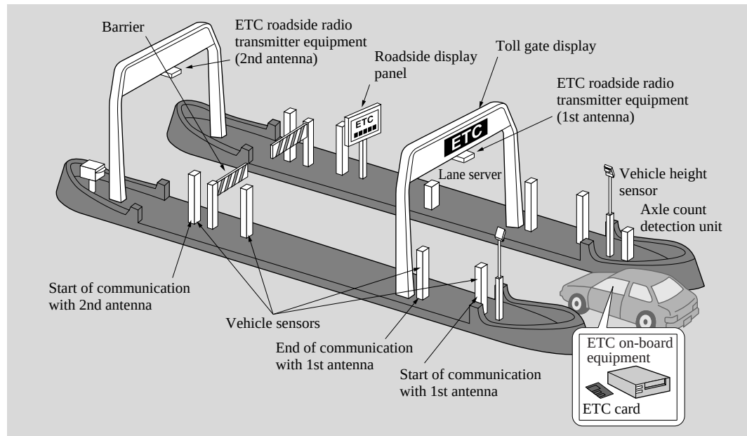
Fig. 2—ETC Device Configuration at Entrance Tollbooth.
