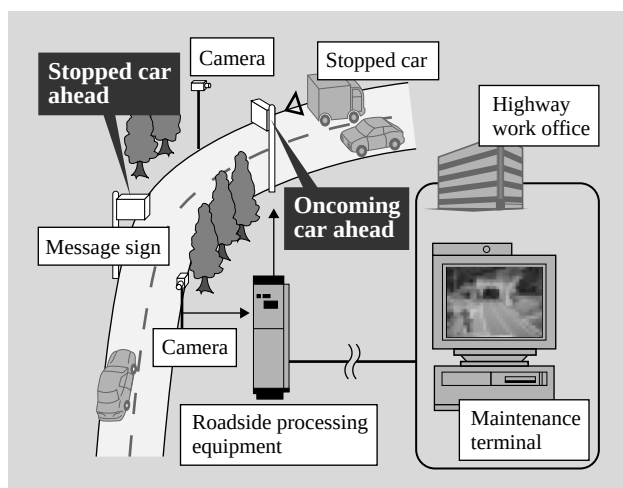
Fig. 4—Typical Configuration of the Danger Warning System. Warns drivers of potential risks ahead when visibility is poor.
