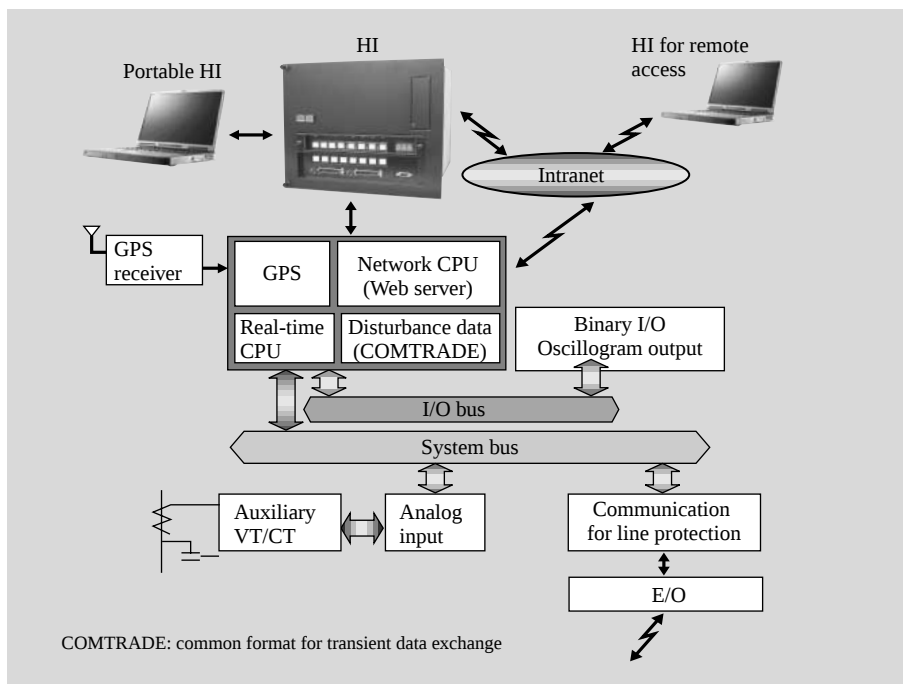
Fig. 4—System Configuration of New Digital Relay Unit. Dual processors for real-time protection/control processing and networking are implemented on a single printed circuit board. This ensures real-time processing performance and flexible accommodation of remote monitoring, control, and analysis over network applications.
