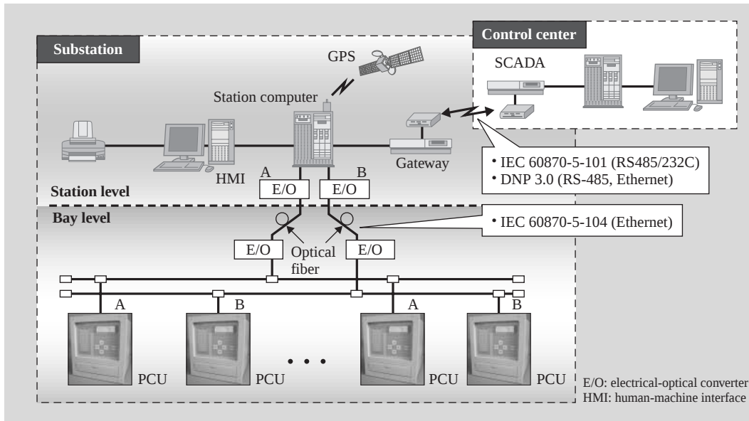
Fig. 3—Overview of Open Network-based Protection and Control System. Remote control and monitoring can be easily implemented by deploying an Ethernet-based IEC communication protocol between bay level in substation and SCADA system in control center.
