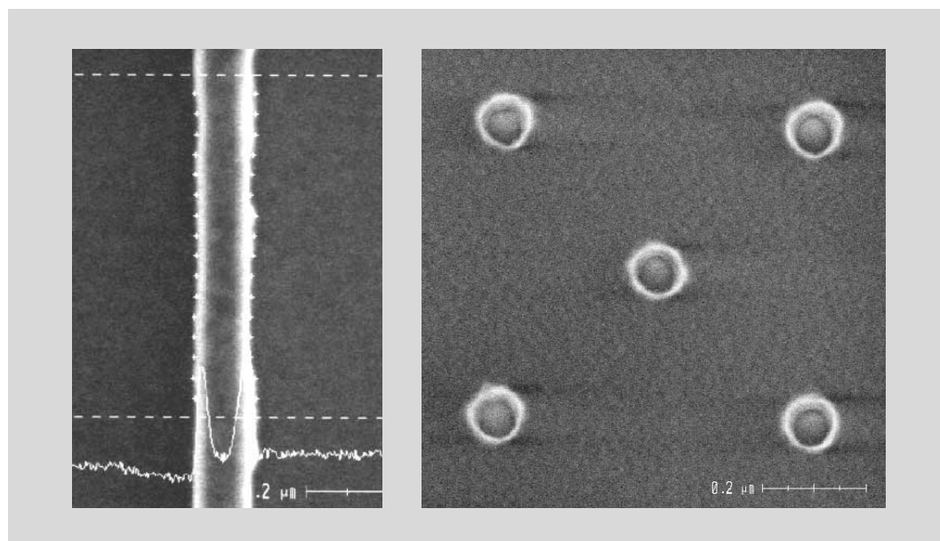
Fig. 2—Examples of Observation of Fine Patterns Using S-9360.
