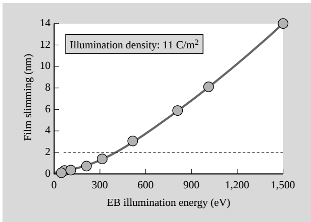
Fig. 8—Example of Slimming Evaluation in Case Where Low-k Film is Illuminated by the EB. This figure shows the relationship between the illumination energy and the degree of slimming. By reducing the illumination energy to 300 eV or less, the slimming can be reduced to 1.4 nm.
