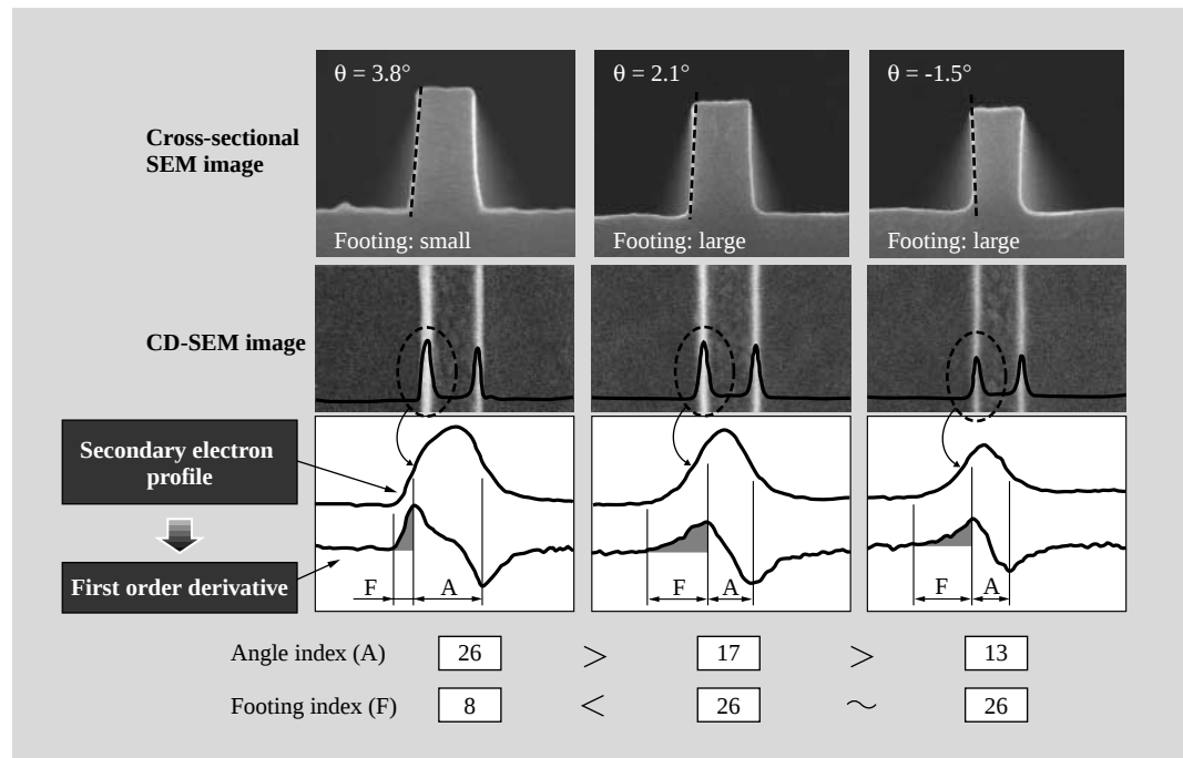
Fig. 9—Examples of Evaluation of Cross-sectional Profile of Gate Pattern Using Etching Process Monitor. The feature quantity of the pattern side wall angle (angle index) and the feature quantity of the bottom part (footing index) can be extracted from the first order derivative of the secondary electron profile.
