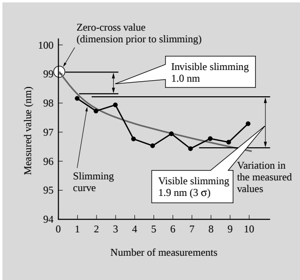
Fig. 4—Reduction of Measured Values Due to Slimming of Resist Pattern.
