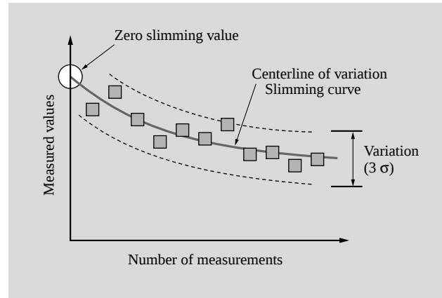
Fig. 6—Example of Measuring Pattern that Slims.
