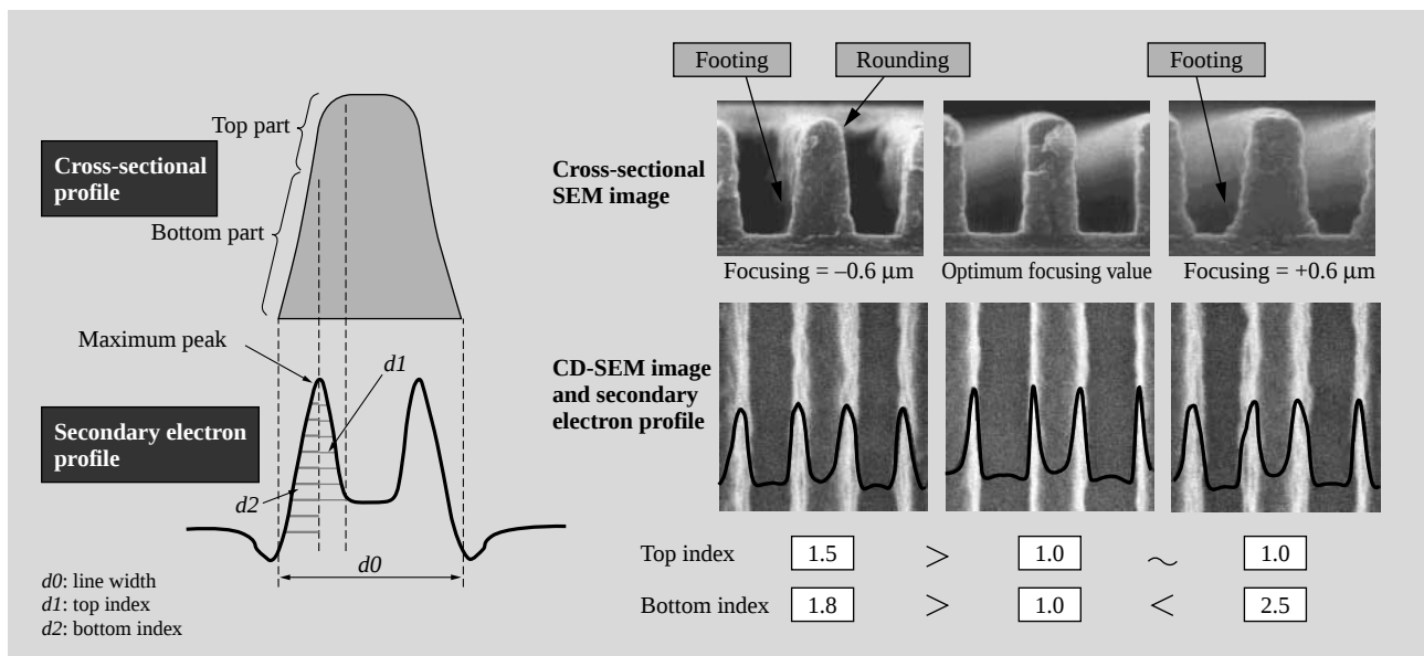
Fig. 10—Focusing Monitor that Uses Top Index and Bottom Index.
