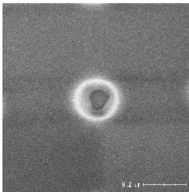
Fig. 3—Example of Observation of High Aspect Ratio Hole Using S-9360.
