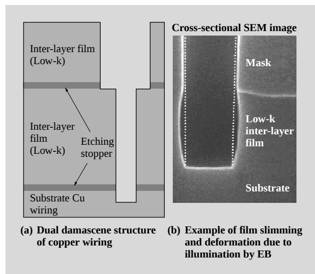
Fig. 7—Example of Cu Wire Dual Damascene Structure and Slimming.
