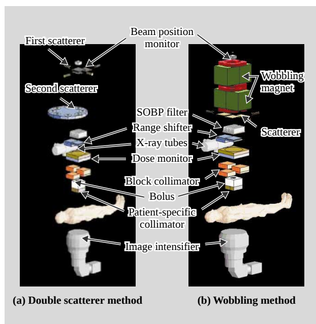
Fig. 4—Configuration of Two Types of Irradiation Nozzle.
