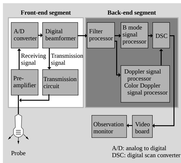
Fig. 6—Overall Block Diagram for Digital Ultrasound Diagnostic Scanner.
