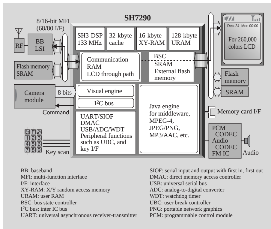
Fig. 3—SH-Mobile1 SH7290 Configuration and System Construction Example.
