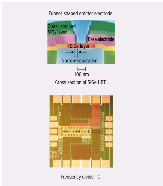
Cross section of SiGe HBT and frequency divider IC
