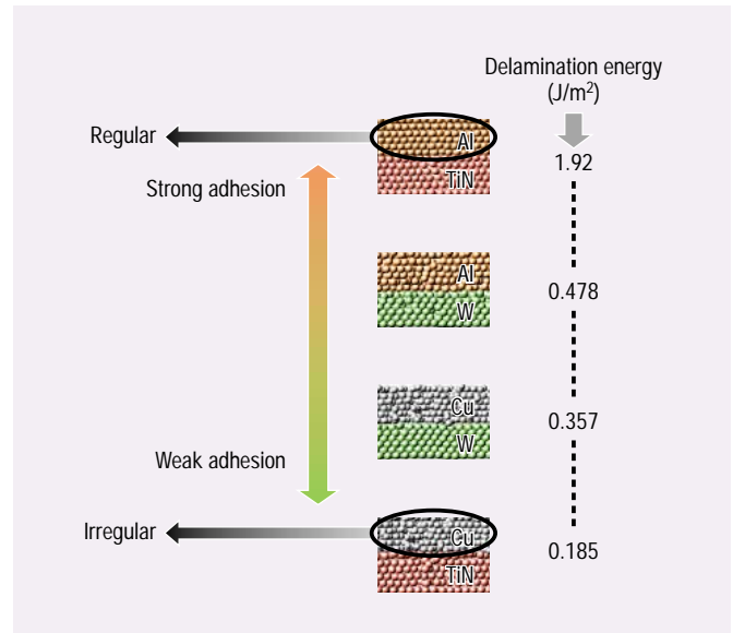
Relationship between delamination energy and configuration regularity obtained from molecular dynamics
