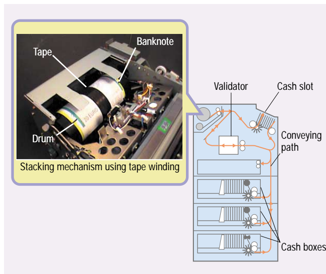
Cash module of Hitachi's HT-2845 ATM
