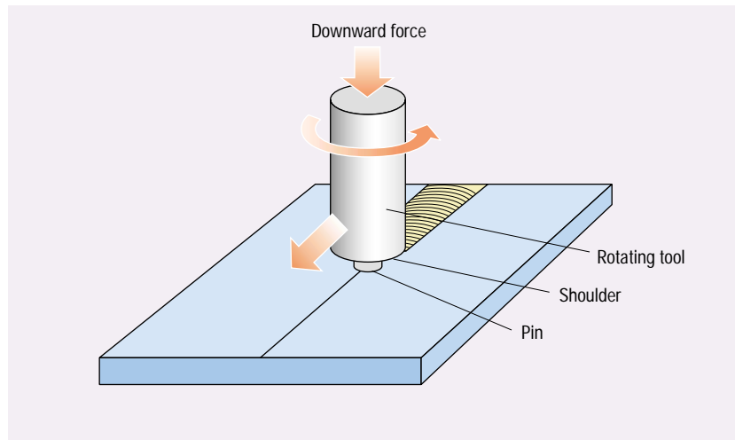
(a) Schematic arrangements illustrating friction stir welding
