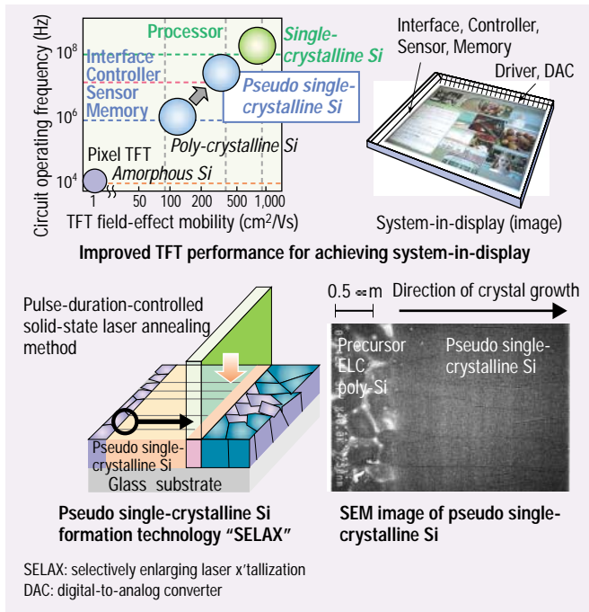
Low-temperature poly-Si TFT formation technology for system-in-display
