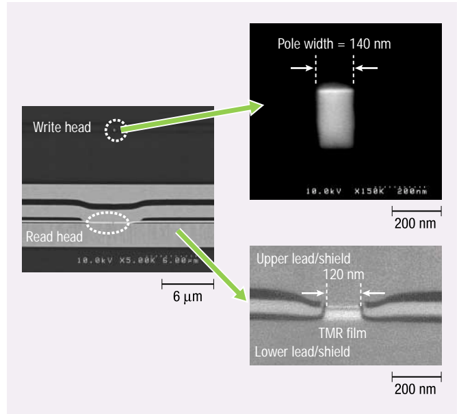
SEM (scanning electron microscope) images of fabricated head observed from air-bearing surface
