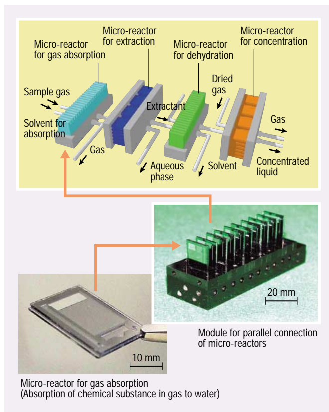
Chemical processing system composed of micro-reactors
