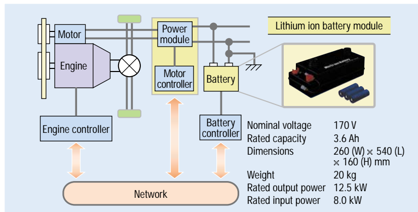
System diagram and lithium ion battery module for HEVs
