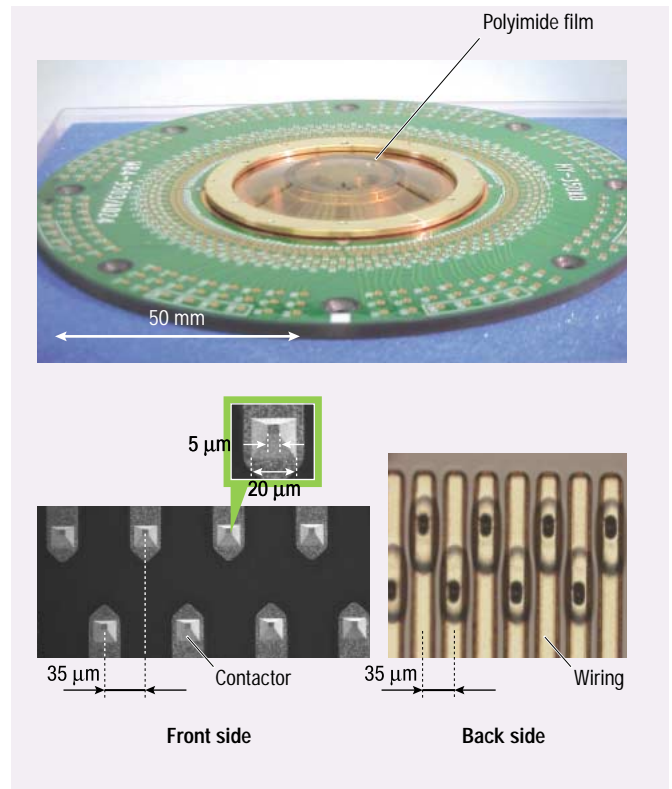
Appearance of the probe card (top), a contactor (lower left), and the wiring (lower right)
