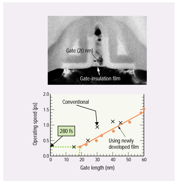
Cross section of 20-nm-gate-length CMOS device (TEM image) (top) and CMOS device (NMOS) operating speed (bottom)
