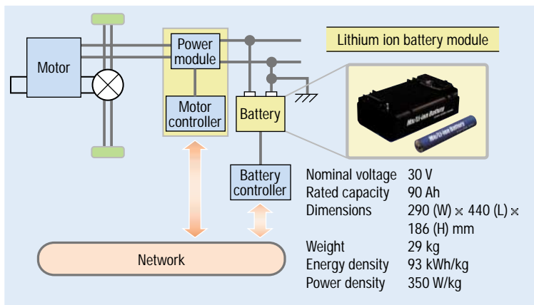
System diagram and lithium ion battery module for EVs
