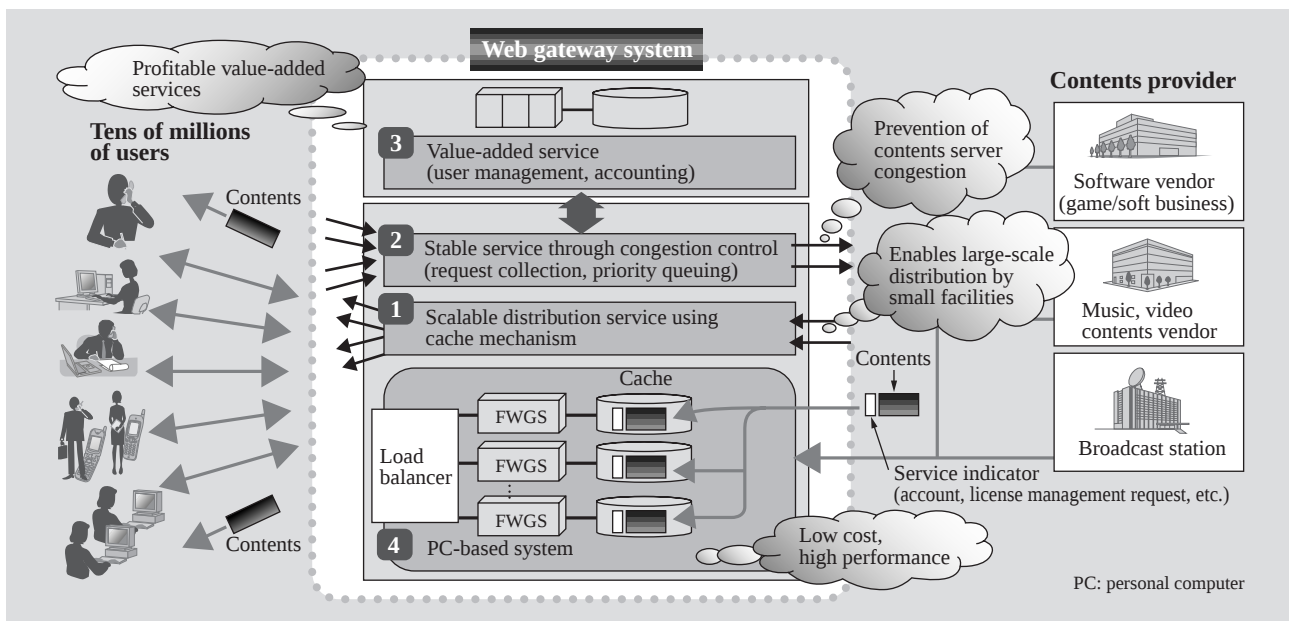
Fig. 2—Web Gateway System.
