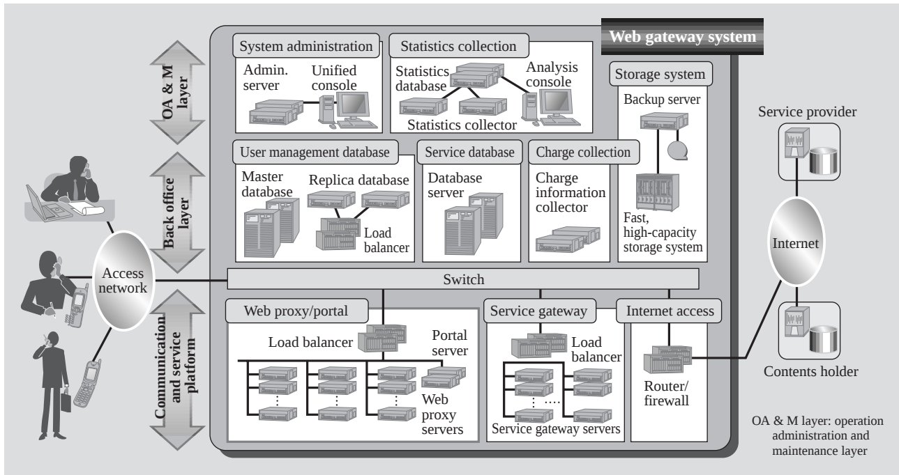
Fig. 1—Web Gateway System Configuration Example.
