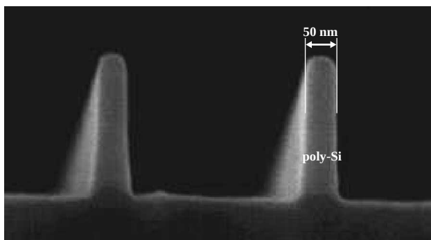
Fig. 7—Formation of a 50-nm Gate.
