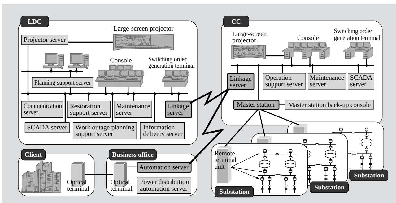
Fig. 2—Example of Information Linkage among SCADA Systems.
