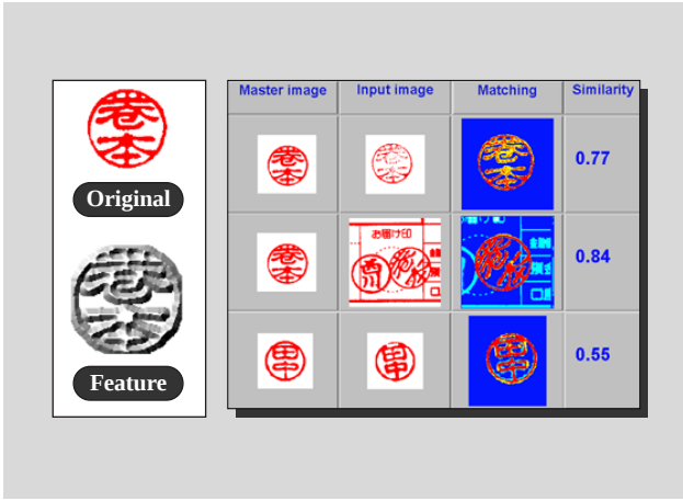
Fig. 9— Seal Similarity Measurement and Verification. Input image is translated and rotated so that it matches the master image.
