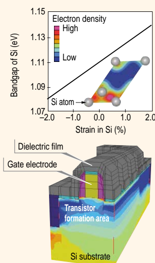
Predicted change in bandgap of Si based on the first principles calculation (top) and analytical result of a three-dimensional strain field in a transistor structure
