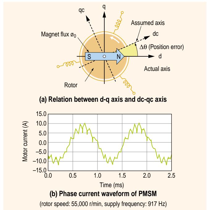
The principle of position sensorless control and the current waveform of PMSM (rotor speed: 55,000 r/min, supply frequency: 917 Hz)
