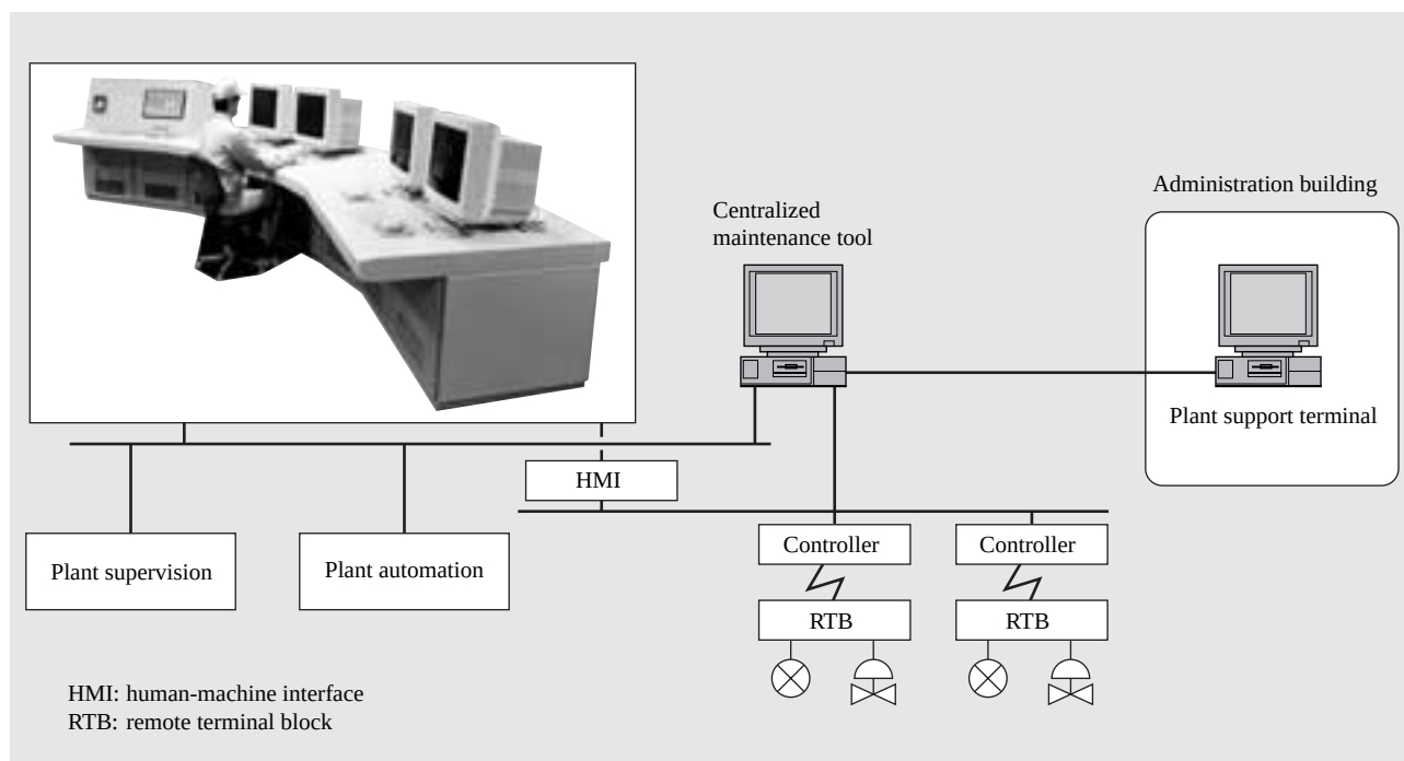
Fig. 2— Example of Configuring the New Supervisory and Control System.
