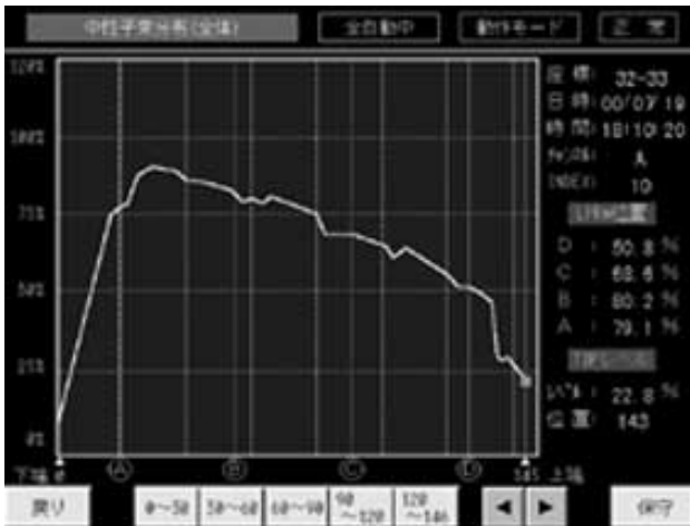
Fig. 4— Screen Shot of Traversing In-Core Probe System (TIP). Replacing the conventional X-Y recorder with a color flat display and digitizing data improves operability and simplifies the management of recorded data.
