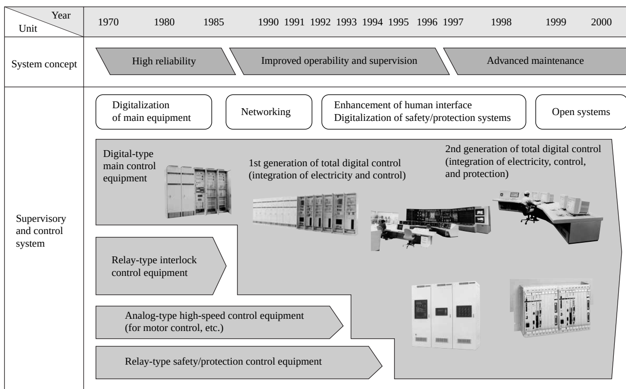
Fig. 1— Evolution of Supervisory and Control Technologies.
