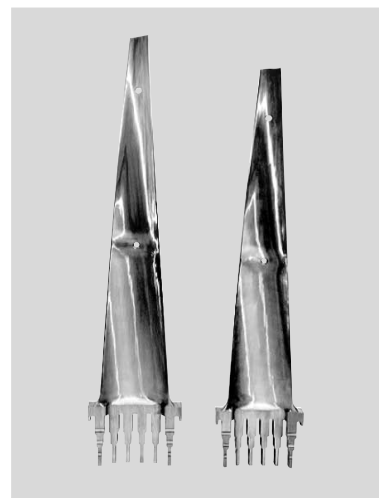
Fig. 1— 52-Inch-Long Blade (Left) and 43-Inch-Long Blade (Right).
