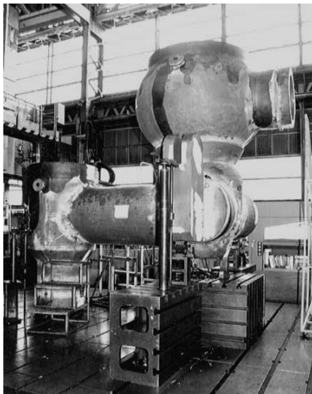
Fig. 4— Main Stop-Valve/Control-Valve Casings. Instead of conventional cast casings, welded-type casings were used to eliminate the possibility of the casings having casting defects and improve the turbine reliability.
