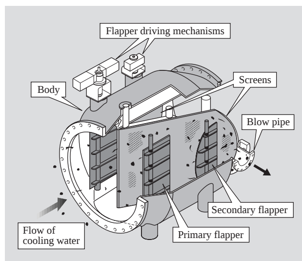
Fig. 6— Filter for Removing Debris.
