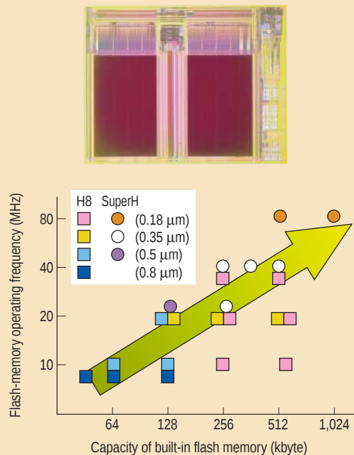
Flash memory to be installed in the 0.18- \mu\text{m} -generation F-ZTAT microcomputer (shown in the picture above), and future development of F-ZTAT microcomputers
