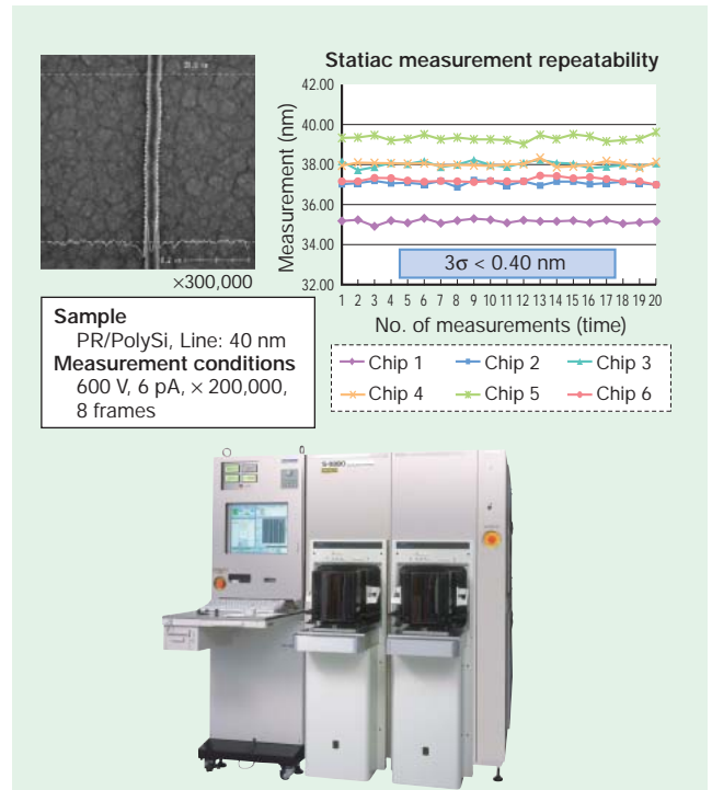
Measured sample, static measurement repeatability (above) and appearance of S-9380 (below)
