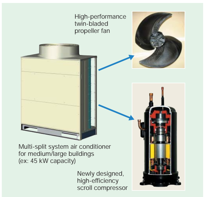
Highly efficient, compact multi-split system air conditioners
