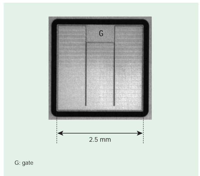
Top view of 2.5 \times 2.5 mm fabricated chip, consisting of 4,486 unit cells
