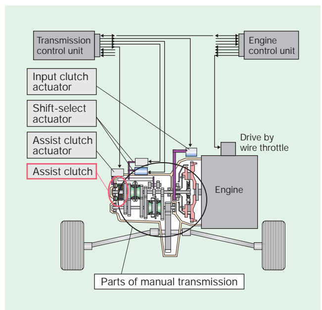
Torque assist automated manual transmission system
