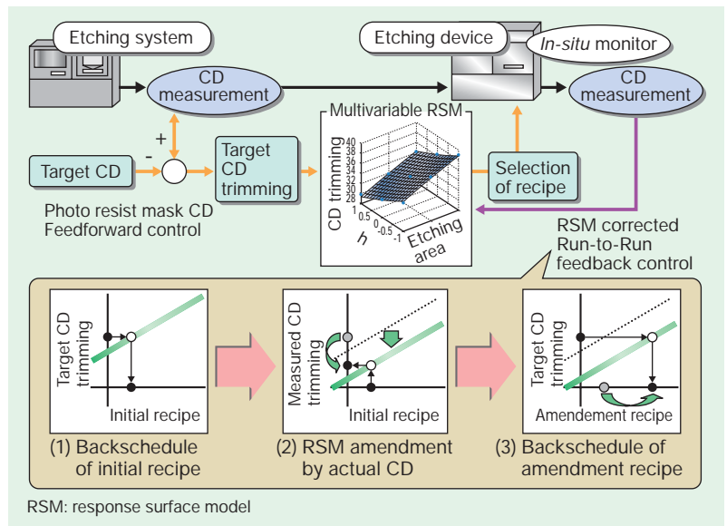
RSM: response surface model Concept of APC techniques with "Run-to-Run Control"
