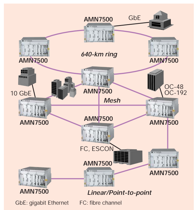
Metro WDM node for next-generation WDM networks
