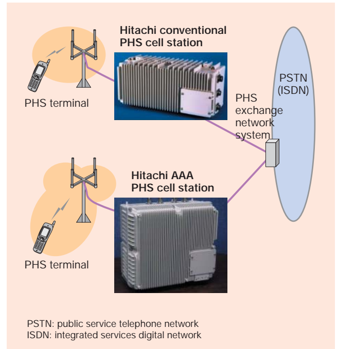
System architecture of PHS cell station
