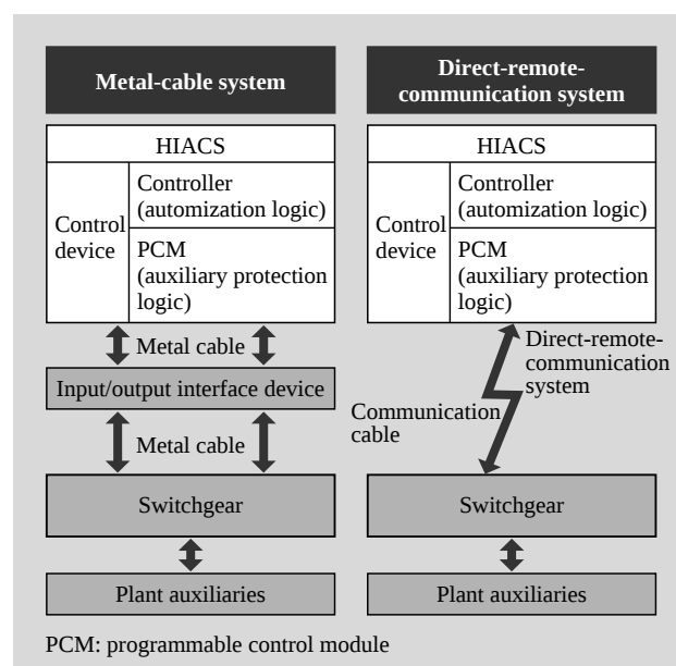
Fig. 6—Interface between Control Devices and Switchgears.
