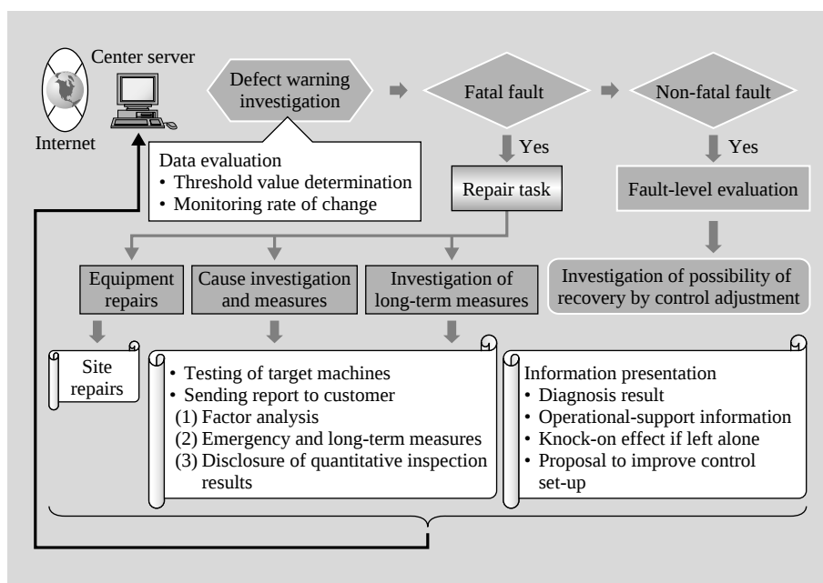
Fig. 6—Process Flow of Monitoring and Diagnosis.
