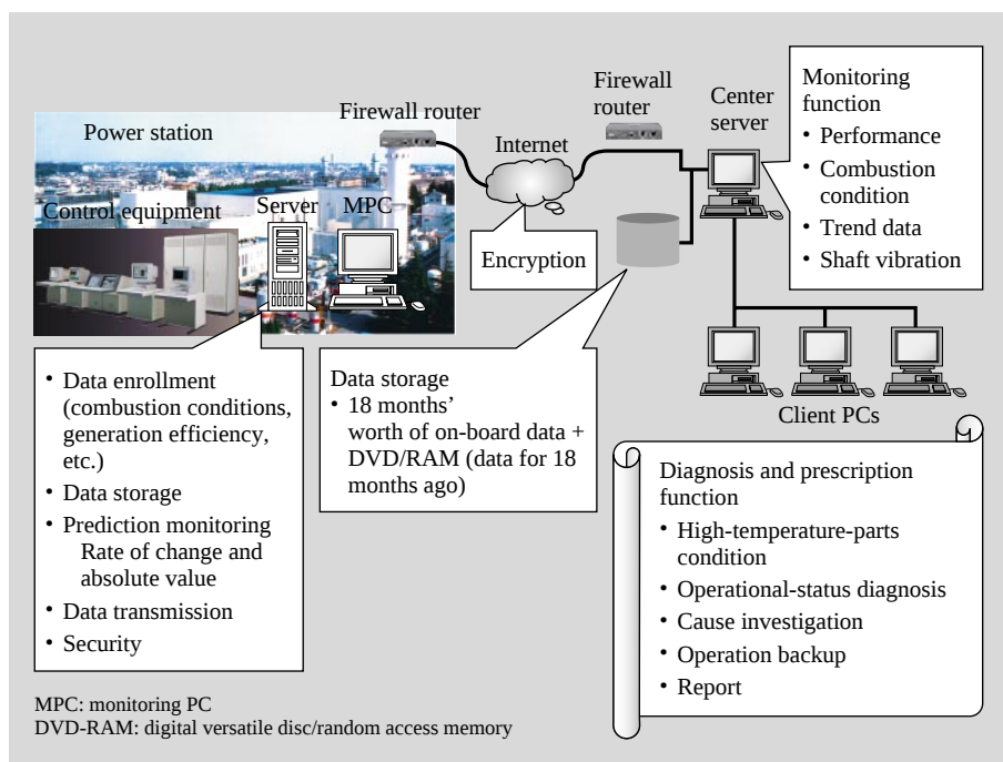
Fig. 5—Overview of Remote-monitoring System.
