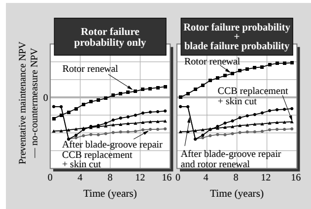
Fig. 3—Example of RBM Evaluation for Maintenance Scenarios Involving Low-pressure Rotor of Aged Steam Turbine.
