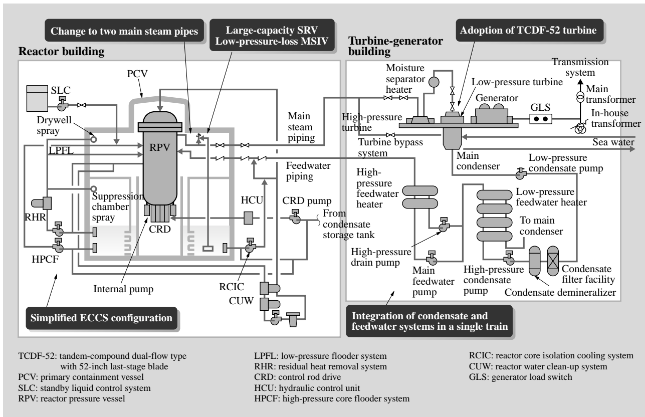
Fig. 3—Newly Developed ABWR Plant Configuration and Features.
