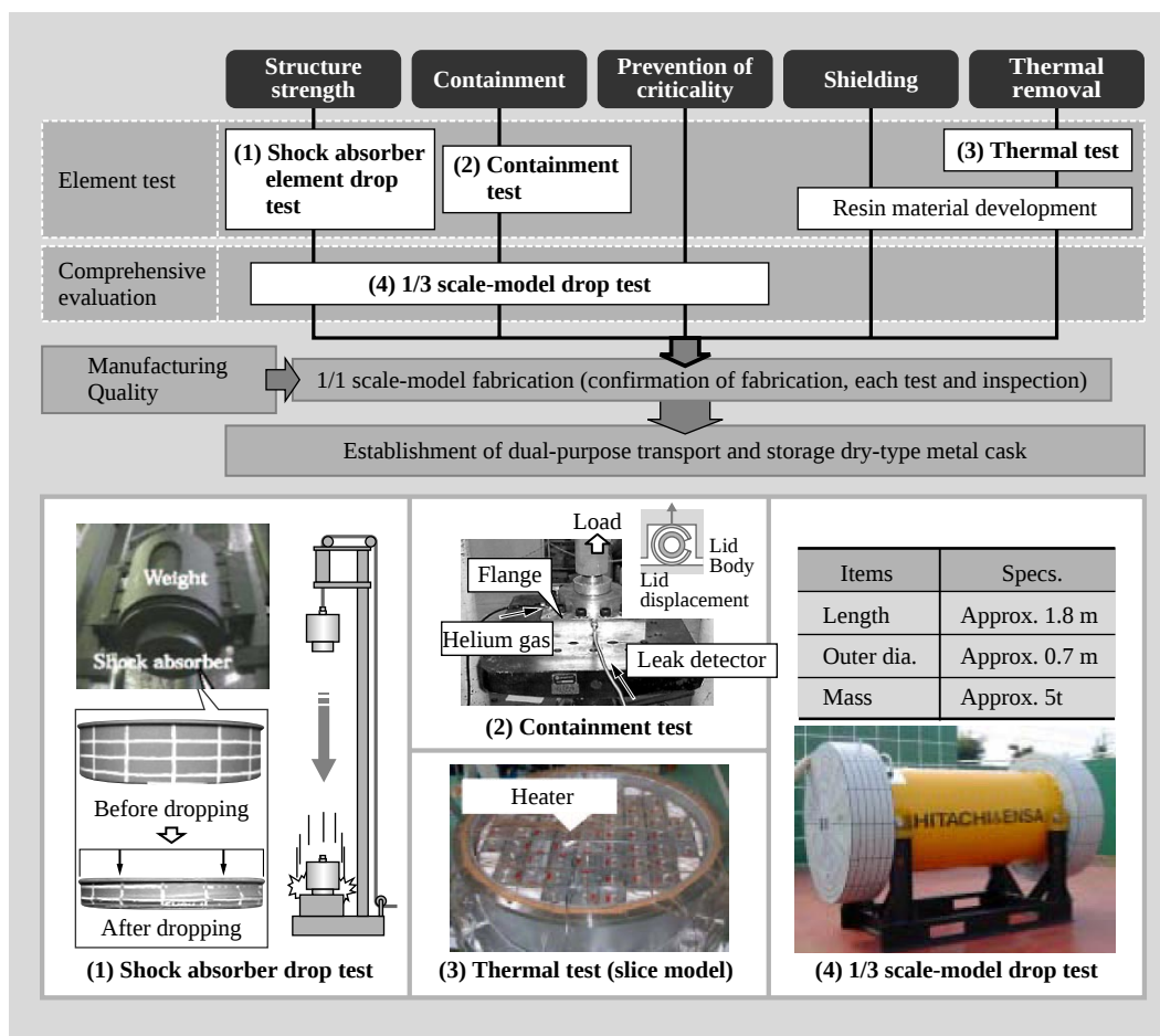
Fig. 5—Development Flow for Dual-purpose Dry-type Metal Cask. Confirmation of safety and establishment of a design method were done through several element tests and a 1/3 scale-model drop test.
