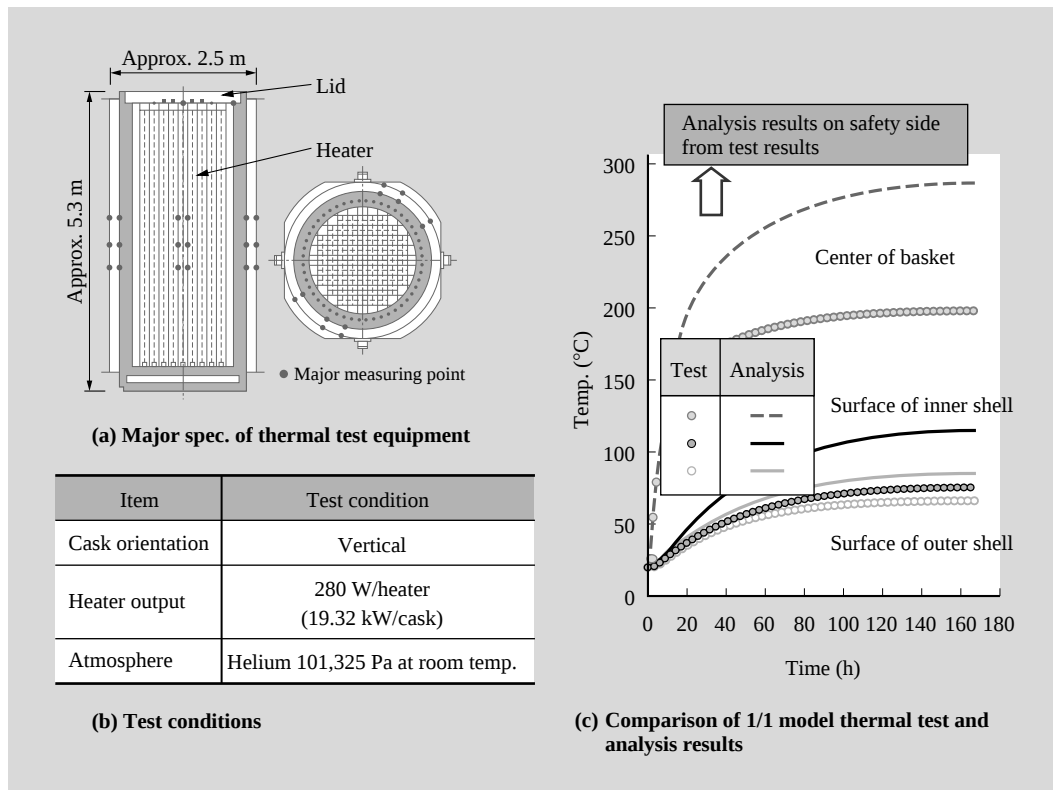
Fig. 8—1/1 Scale-model Thermal Test Conditions and Outline of Results. We found that the temperature in parts of the actual cask was below that permitted and the spent fuel temperature was well below 300°C providing a sufficient margin.
