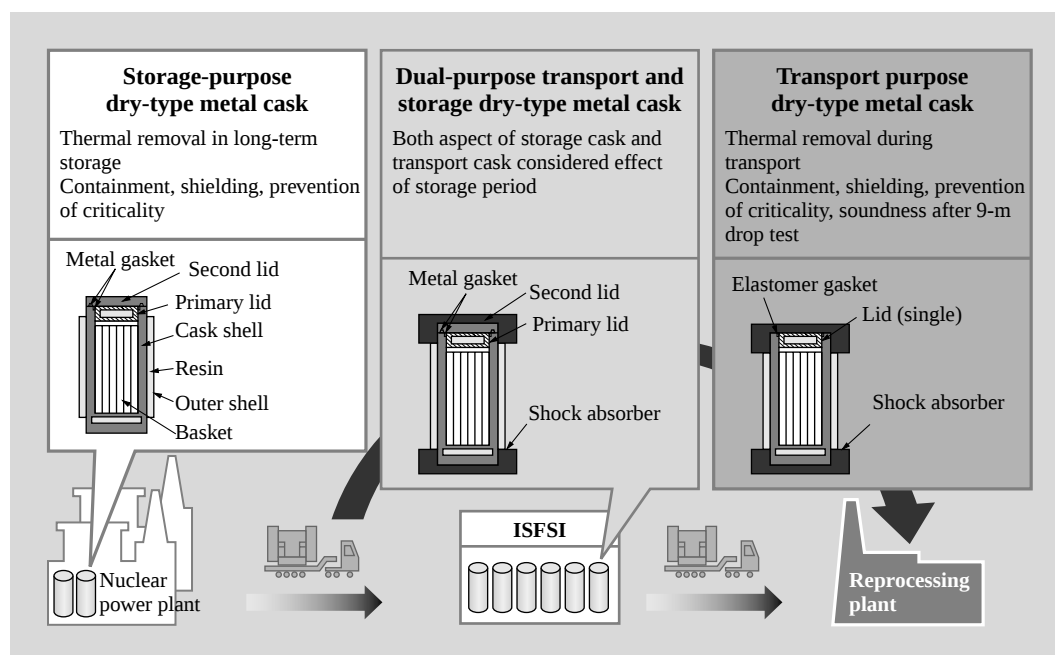
Fig. 2— Characteristics of Dual-purpose Transport and Storage Dry-type Metal Cask. Design with considering storage before and after transport is required.
