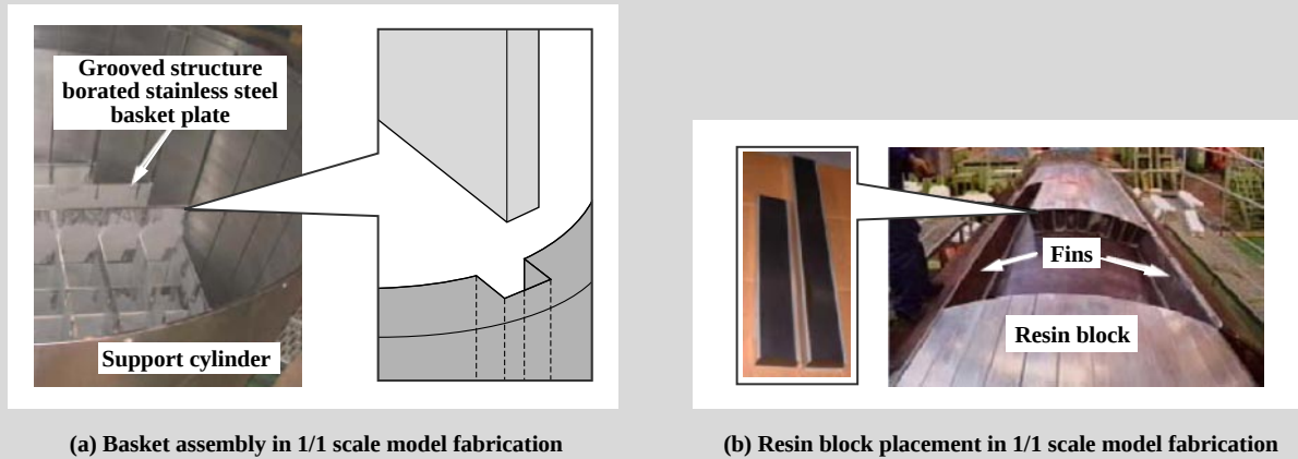
Fig. 4—Outline of Basket Structure (a) and Resin Block Structure (b). To improve reliability and reduce fabrication costs, grooved and block structures were adopted.
