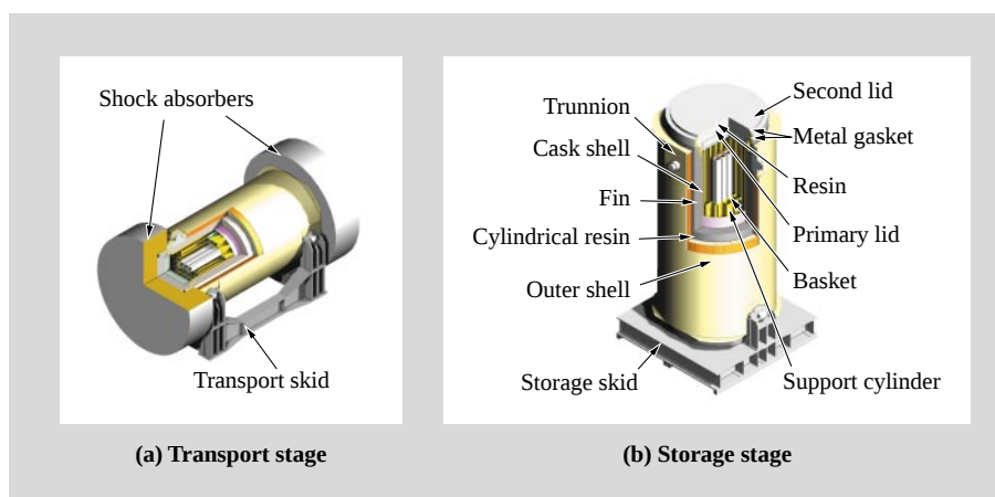
Fig. 3—Outlines of Developed Dual-purpose Transport and Storage Dry-type Metal Cask. 69 bundles of BWR fuel (Step I, 10- year cooling) can be loaded. Its length is approx. 5.5 m and outer diameter is approx. 2.5 m. Mass is approx. 130 t during transport and approx. 120 t in storage.
