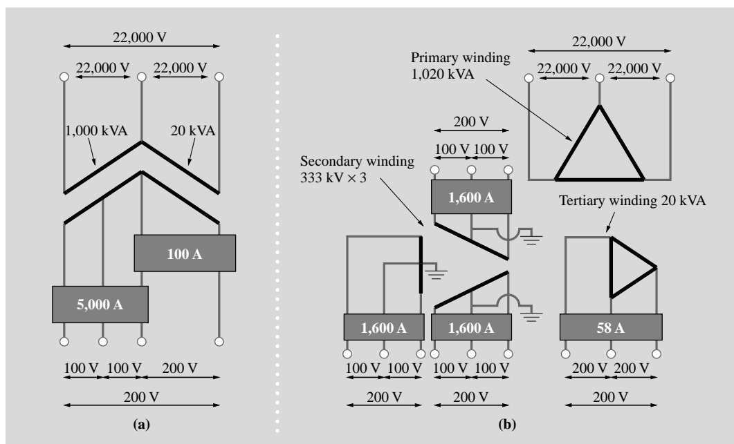
Fig. 8—Comparison of Transformer Cables.
