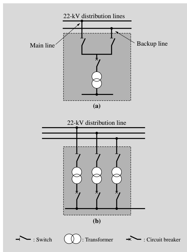
Fig. 2—Schematic Single-line Connection for Distribution Systems.
