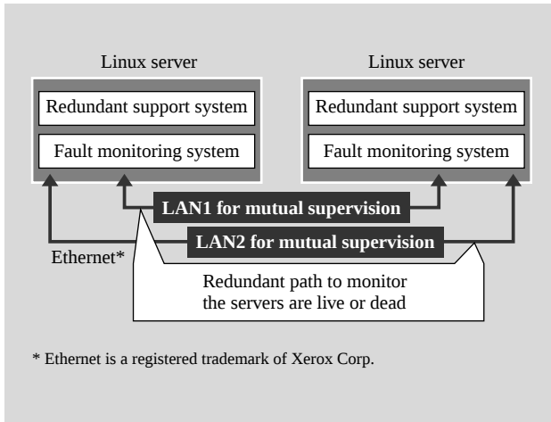
Fig. 4—Server Redundant Support System.
