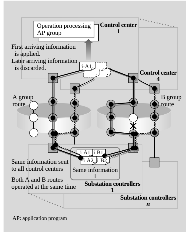
Fig. 5—Schematic of Transmission Protocol.
