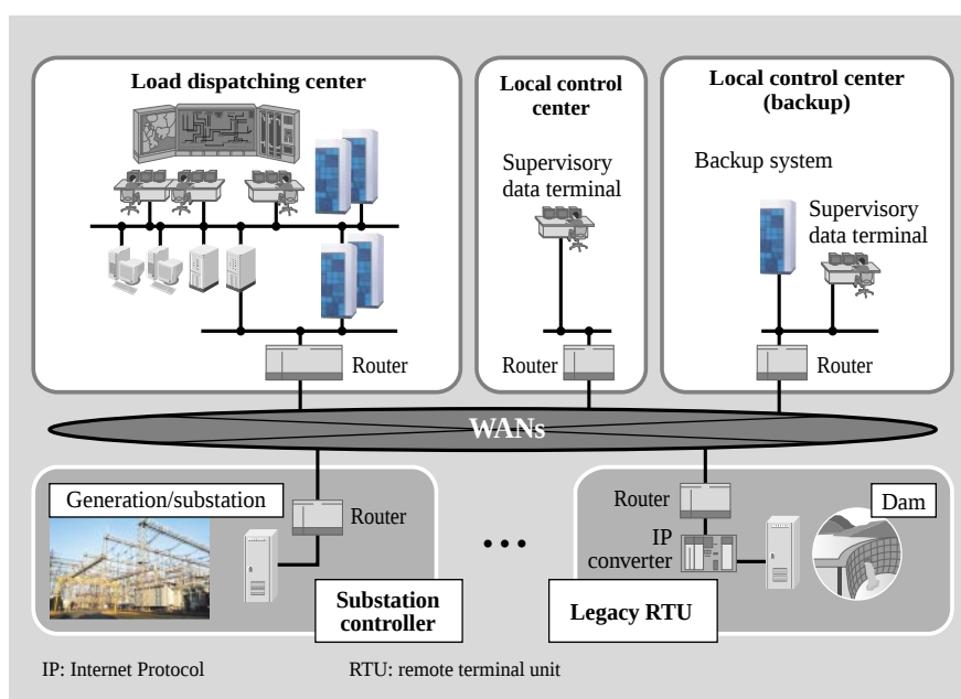
Fig. 1—Configuration of Load Dispatching Control System, The Kansai Electric Power Co., Inc.'s Plant in Tokai Region.
