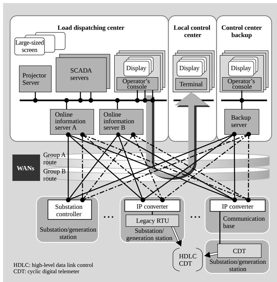
Fig. 2—Configuration of WANs-interconnected SCADA systems. Substation controllers are linked to higher stations by a broadband network.
