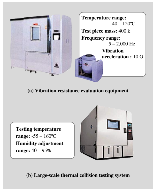
Fig. 11—Endurance Testing Equipment. Equipment and evaluation conditions for evaluating vibration and thermal collision reliability.
