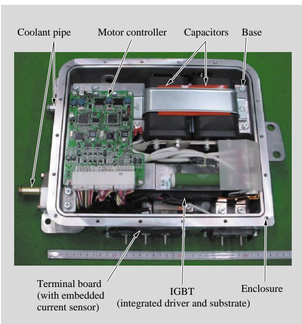
Fig. 8—Inside 5th-generation Inverter. Size and weight reduction can be achieved using direct water-cooled IGBT twin inverter.
