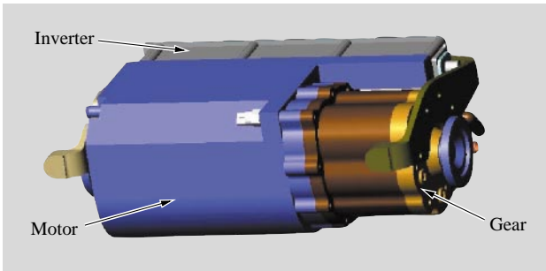
Fig. 9—Integrated Electrical-mechanical Unit for HEV Drive. The system as a whole can be significantly reduced in size and cost by integrating the motor, inverter, and gear.
