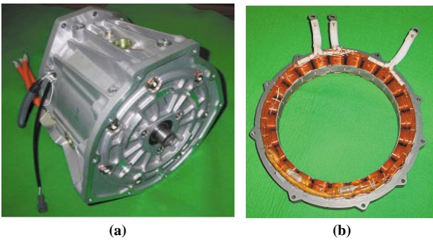
Fig. 3—100 kW-class Motor (a) and Thin Profile Motor (b). Prototype models of motors are under development that are smaller and lighter yet provide higher output.
