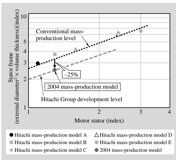
Fig. 4—HEV Motor Downsizing Level. Motor frame has been downsized by 25% while motor torque remains unchanged.
