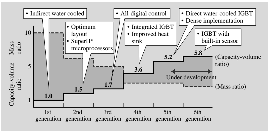
Fig. 7—Inverter Trend. Inverters are becoming progressively smaller and lighter, and the technologies enabling this development are shown.
