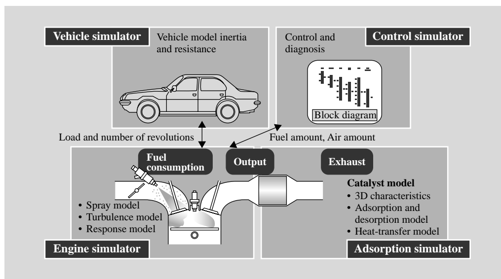
Fig. 5—Integrated Simulation Environment for Development of Engine-control Technologies. Establishing an integrated simulation environment — covering atomization behavior within the engine up to vehicle driveability — has resulted in reduced development times and improved system performance and reliability.
