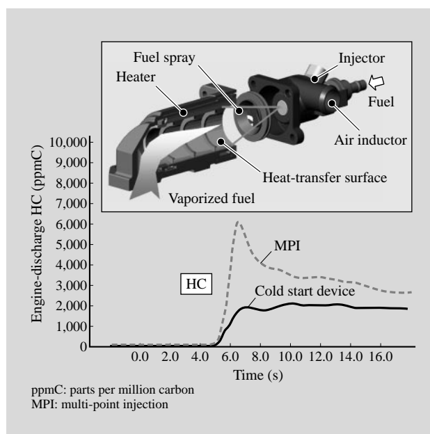
Fig. 2—Cold Start Device Structure and Test Results on Real Vehicle.
