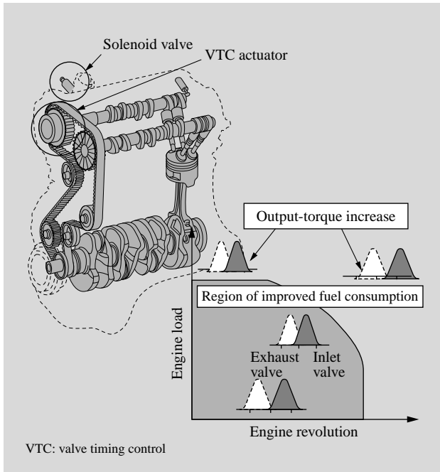
Fig. 3—Design Features and Structure of Variable-valve-control System. The system is designed to optimize the target engine by means of various kinds of actuators and mechanisms.
