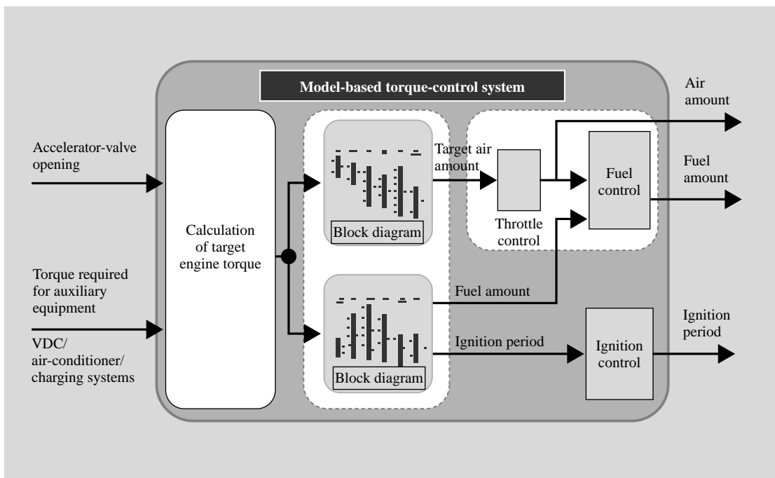
Fig. 4—Block Diagram of Torque-based Control. The torque-based control system enables precise cooperation between the drive-train and chassis systems.
