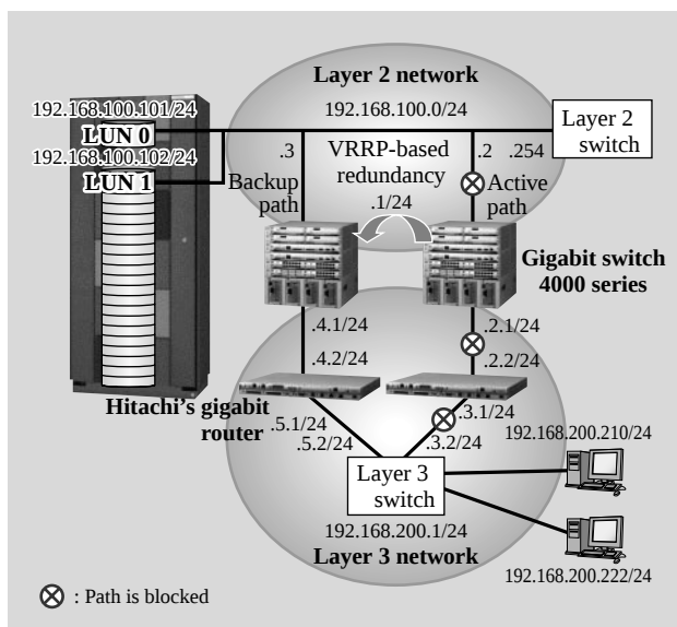
Fig. 4—Example of Storage Redundancy Implemented with VRRP.
