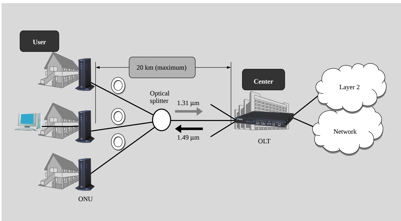
Fig. 2—Basic Configuration of Gigabit Ethernet PON.
