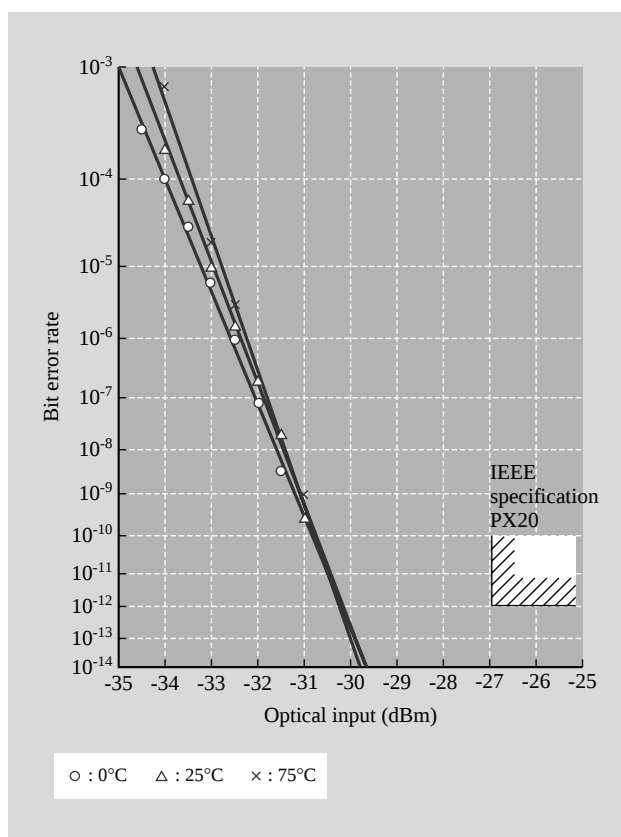
Fig. 3—Reception Characteristics of the OLT for Optical Burst Signals.
