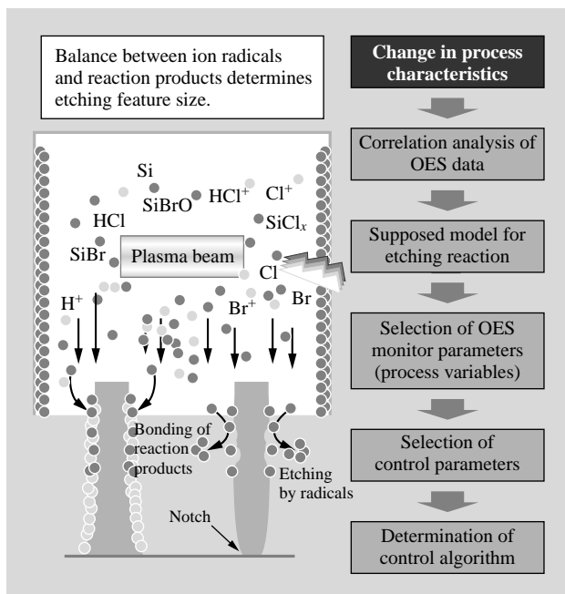
Fig. 3—Etching Reaction Model and Flow for Determining Control Algorithm.
