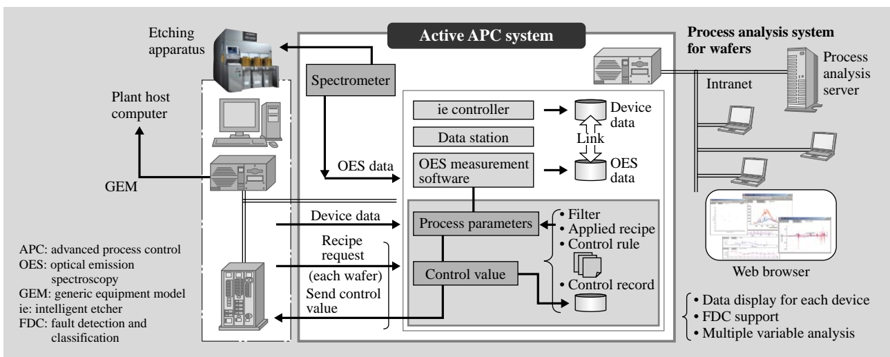
Fig. 1—Overall Composition of High-accuracy Etching System with Active APC Capability.
