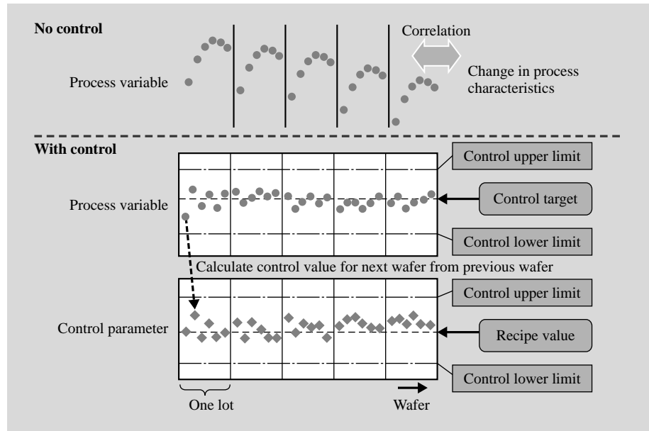
Fig. 4—Execution Concept of Active APC. In the control method, the deviation between the previous process-monitoring results and the target value is determined, and the conditions for the next etching are set according to that deviation. This procedure is called “run-to-run” control.
