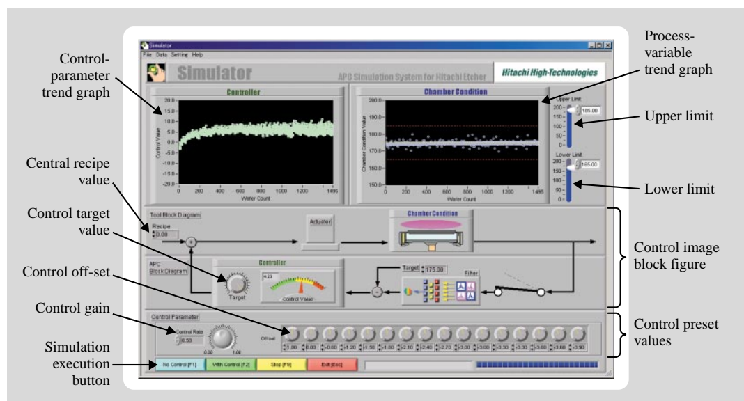
Fig. 5—Active APC Simulation. Before actual active control is executed, the optimum control constants can be obtained by simulation.
