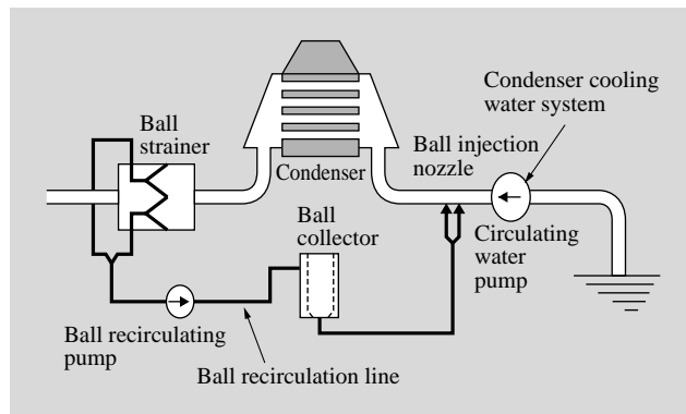
Fig. 2—Basic Structure of Tube Cleaning System.
