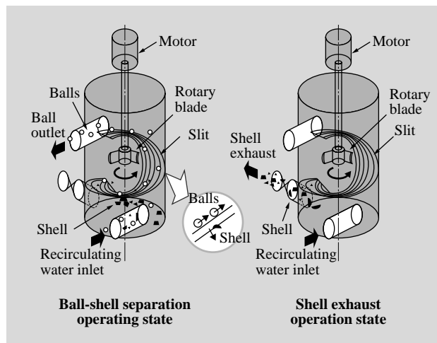
Fig. 5—Principle of Ball-shell Separator.
