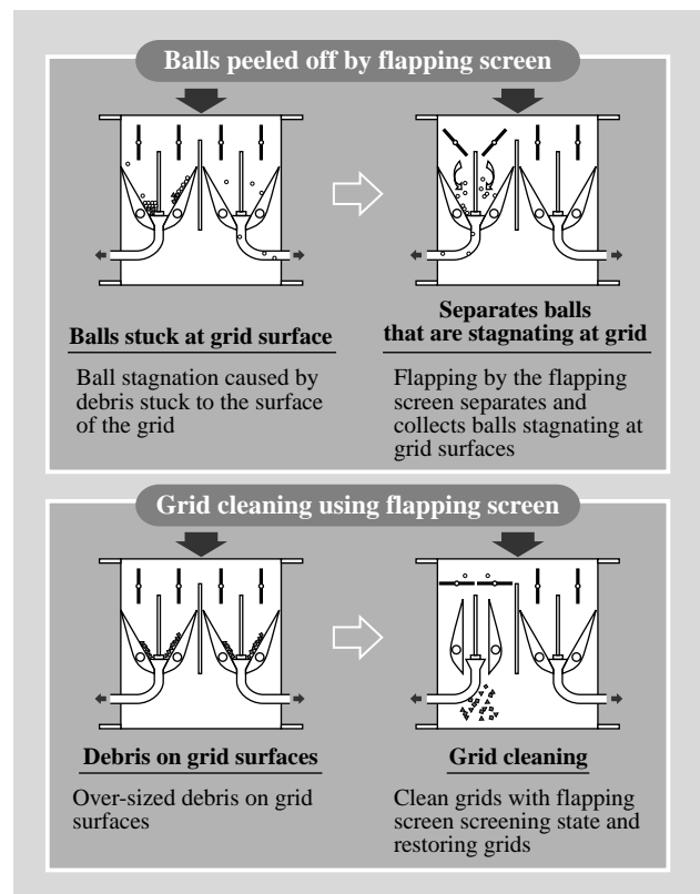
Fig. 4—Operating Principle of Ball Strainer with Flapping Screen. Flapping of the flapping screen collects cleaning balls stuck at the screen and cleans grids.
