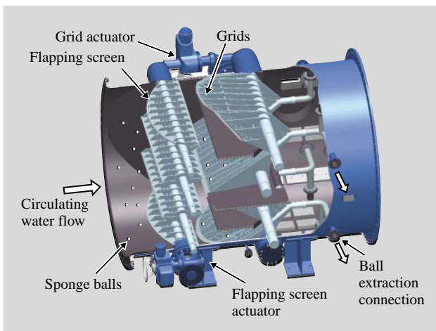
Fig. 3—Overview of Ball Strainer with Flapping Screen. A high-performance ball strainer is implemented by mounting a flapping screen on the upstream side of a conventional ball strainer.
