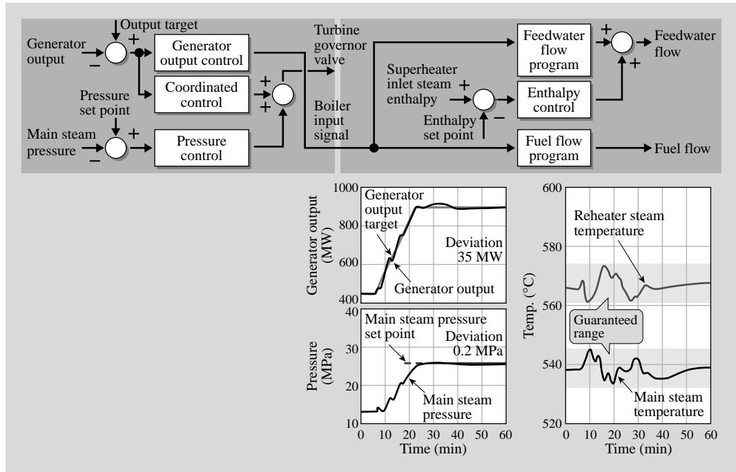
Fig. 6—Coordinated Control Scheme. Disadvantages of “boiler follow control” and “turbine follow control” are corrected by adding compensation to both the turbine and boiler control based on the “turbine follow control.”
