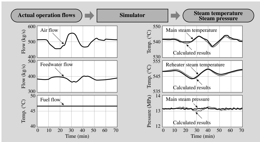
Fig. 8—Simulator Verification Using Site Commissioning. Actual plant process behavior closely corresponds to the plant behavior predicted by developed simulator.
