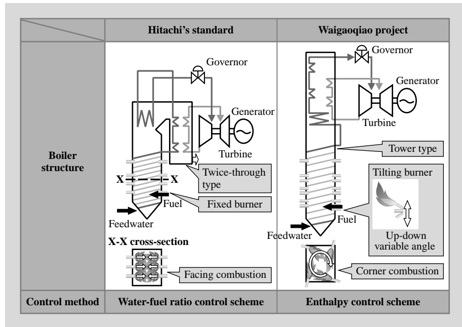
Fig. 3—Comparison of Hitachi and Waigaoqiao Project Boilers. The boilers are substantially different in structure, combustion method, and control method.
