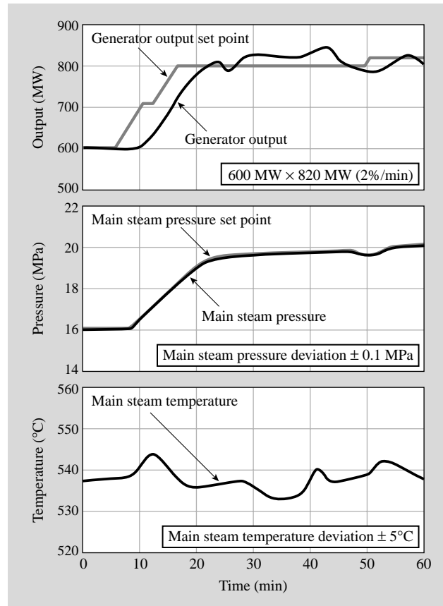
Fig. 7—Example Trial Operation Results. Main steam pressure and temperature satisfy the control performance specifications as predicted by the simulation analysis.
