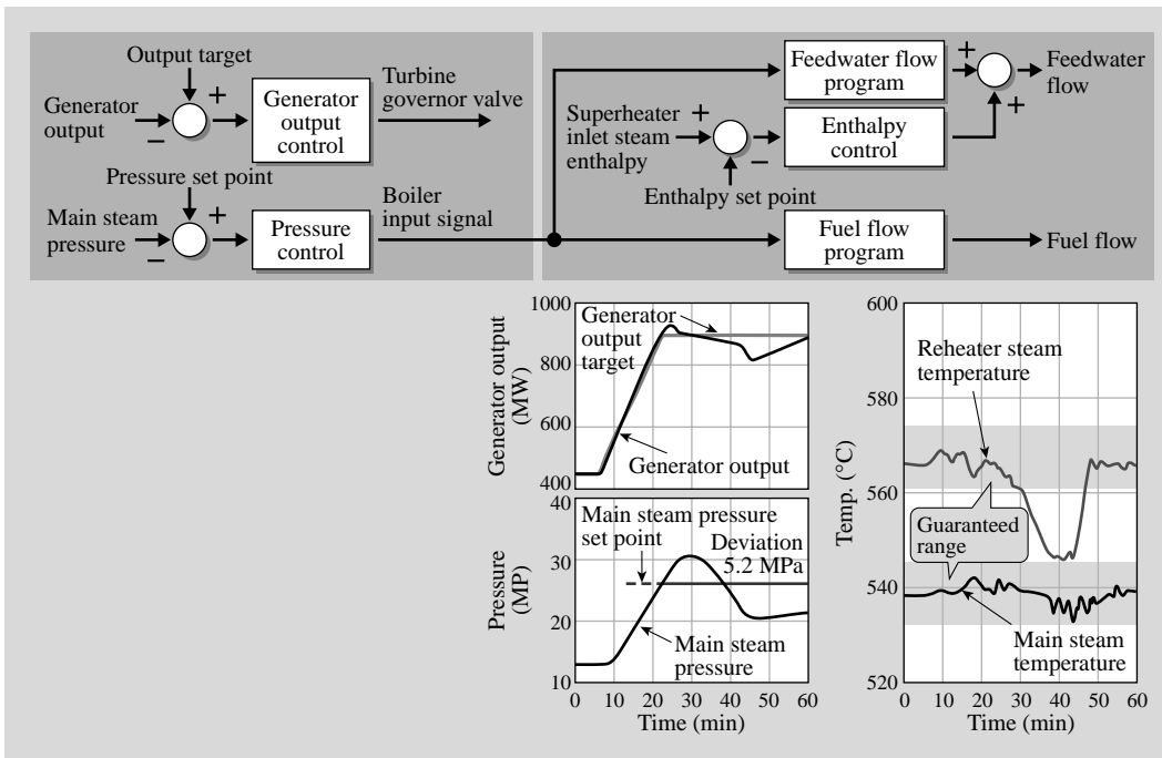
Fig. 4—Boiler Follow Control Scheme. Generator output is controlled by the turbine and main steam pressure is controlled by the boiler.
