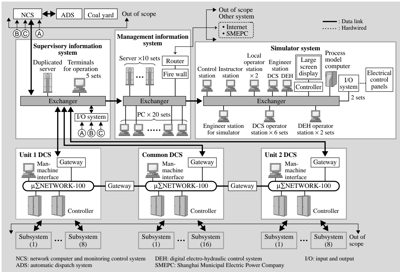
Fig. 2—Overall System Configuration of the New-generation Integrated Monitoring and Control System. All DCSs, SISs, MISs, and subsystems are organically interconnected by a high-speed, large-capacity network.
