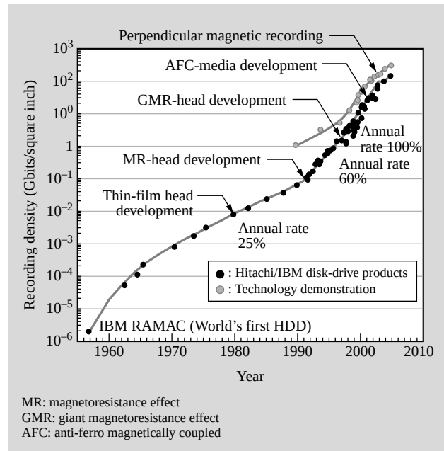
Fig. 2—History of Increasing Recording Density. Since the world’s first HDD appeared in 1956, its recording density has been steadily increasing.
