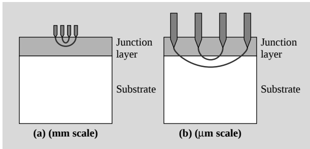
Fig. 8—Schematic of Ultra-shallow Junction Measurement Using a 4-point Probe.
