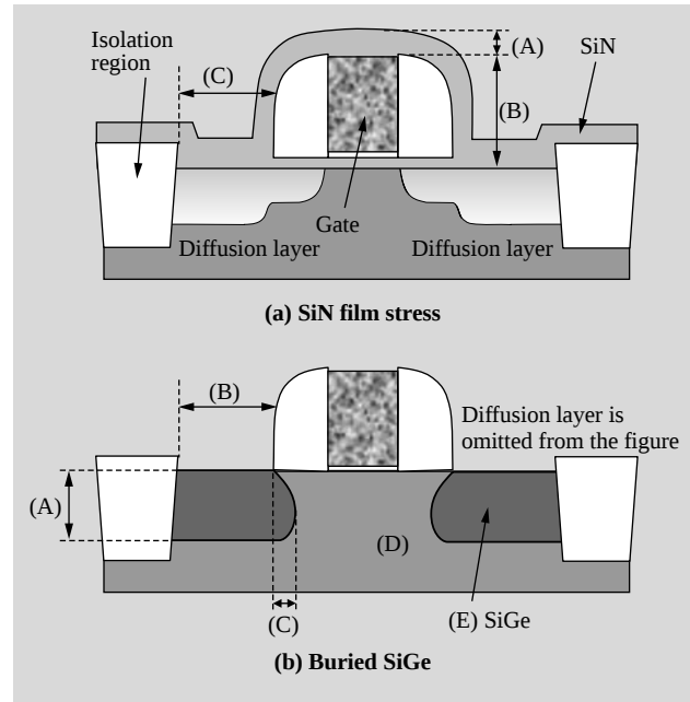
Fig. 4—Dimensions Affecting Stress Magnitude Using External Stress Technology.
