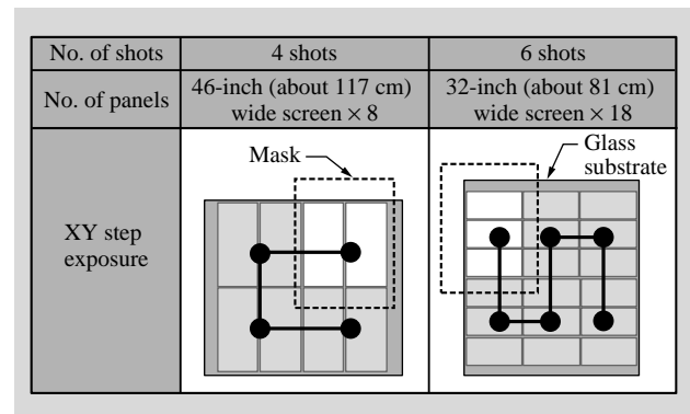
Fig. 6 — Examples of Panel Layouts.
