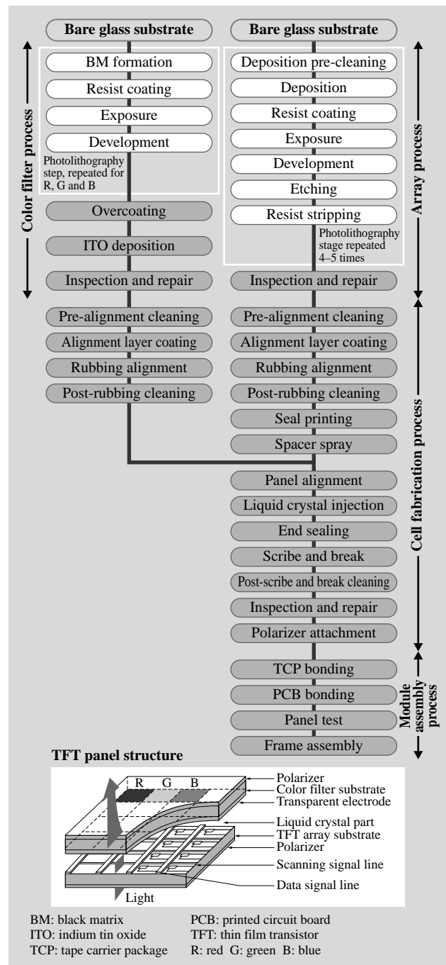
Fig. 3—TFT LCD Fabrication Stages and Panel Structure. The TFT LCD fabrication process consists of an array process, a color filter process, a cell fabrication process, and a module assembly process.
