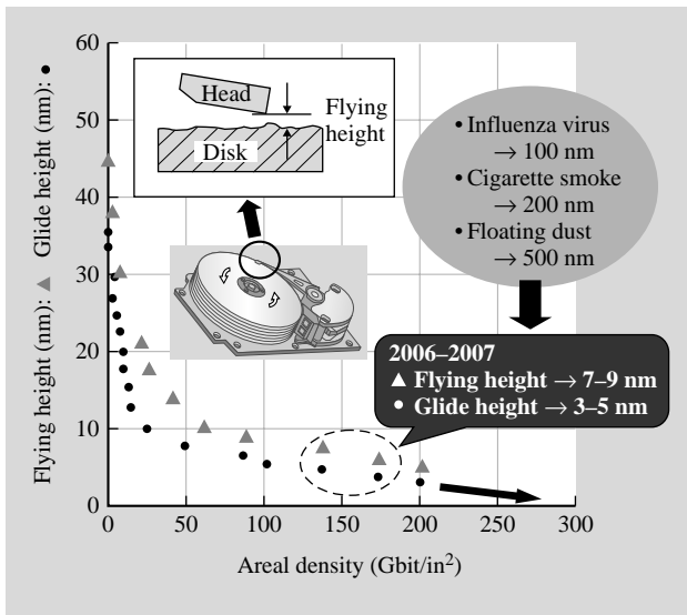
Fig. 8—Glide Height and Flying Height as Function of Surface Recording Density.
