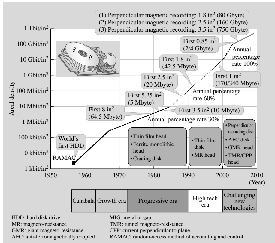
Fig. 2—Transitions in HDD-areal Density and Interent Technologies. Since the world’s first HDD appeared in 1956, improvement of its areal density has continued unabated. Up until 1990, areal density grew annually by 30%, and after that time, it grew even faster, namely, by more than 60% annually. Such growth was accomplished by application of new technologies like MR and GMR head and high-density-storage disks. Likewise, from now onwards, the introduction of new technologies looks likely.
