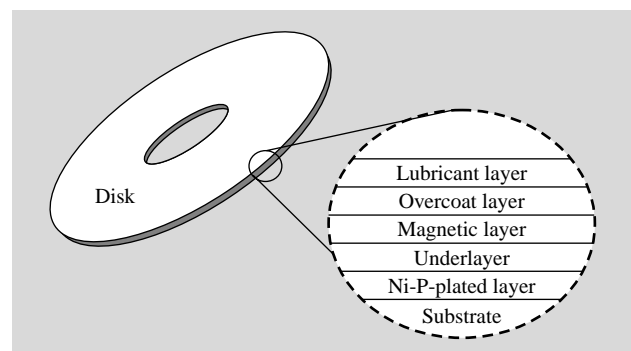
Fig. 3—Disk Cross-sectional Structure (One Side).
