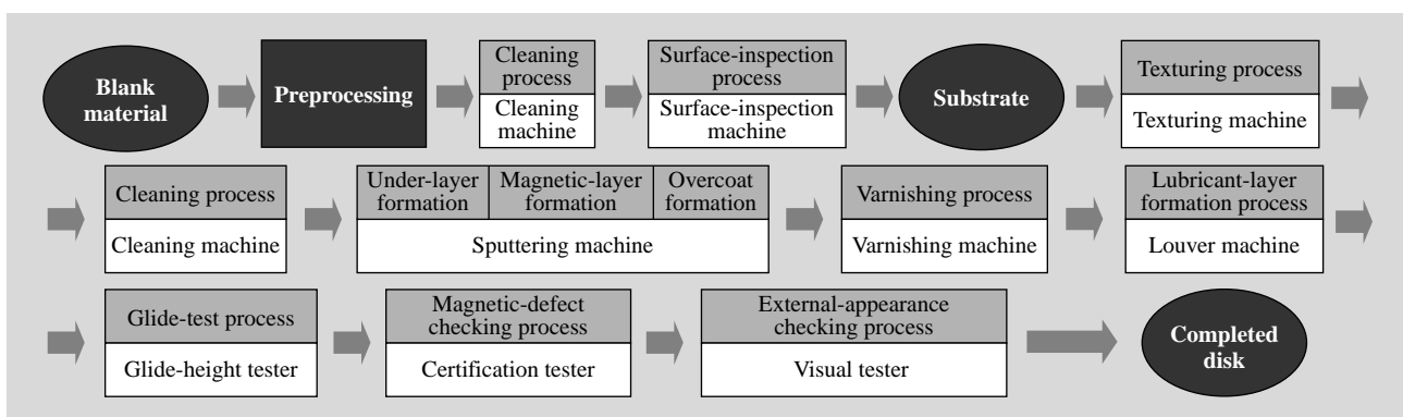
Fig. 4—Substrate and Disk-fabrication Processing.
