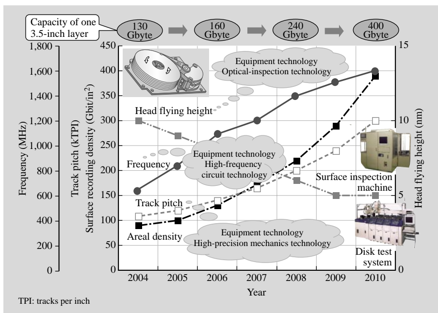
Fig. 1—HDD Technology Roadmap and Facility Technologies. The main facility technologies for handling measurement of the parameters in the main specifications of HDDs, namely, surface recording density, track pitch, head flying height, and frequency, are shown.
