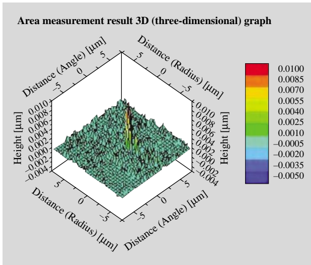
Fig. 14—An Example of Shape Analysis of Minute Defects by Interferometry Optics.
