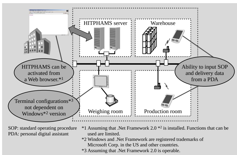
Fig. 1—New Functions and Features of Manufacturing Execution System HITPHAMS Version 2.0. The new version HITPHAMS can be accessed from a Web browser, is no longer dependent on Windows OS (operating system) version, supports SOP entry from PDAs, and permits entry of delivery control data.
