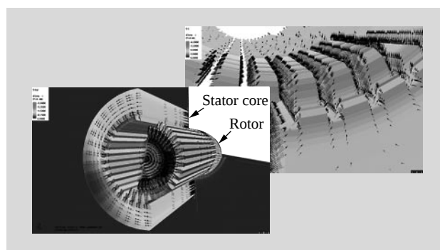
Fig. 4—Three-dimensional Magnetic Field Analysis. Structure around the stator core is optimized through detailed analysis of magnetic flux around the stator core and generator losses.
