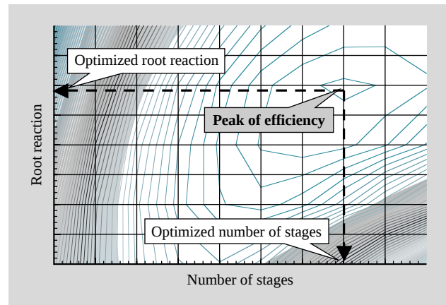
Fig. 2—Optimization Example of Steam-path Design.
