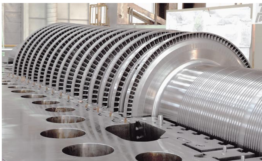
Fig. 1—High-pressure Turbine Unit of the 200-MW Steam Turbine for the Kwangyang Combined-cycle Power Plant of Republic of Korea's K-Power. The high-pressure turbine rotor is integrated in the lower half of the turbine casing, and the high-pressure turbine adopts optimized reaction blades (newly developed by Hitachi) for all turbine stages.
