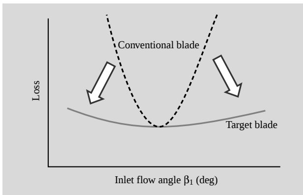
Fig. 4—Profile-loss Characteristics.
