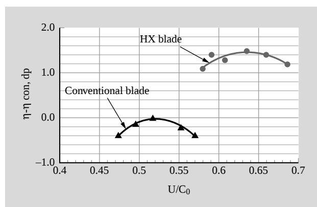
Fig. 7—Comparison of Stage Efficiency of Conventional and HX Blades.
