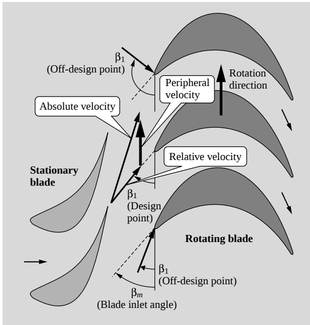
Fig. 3—Velocity Triangles.
