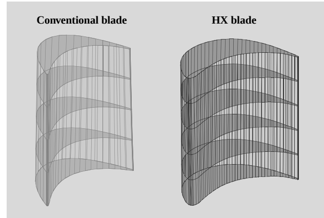
Fig. 5—Comparison of Profiles of Conventional Blade and HX Blade.
