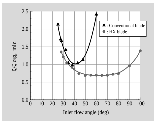
Fig. 6—Comparison of Inlet Flow Angle Characteristics of Conventional and HX Blades.
