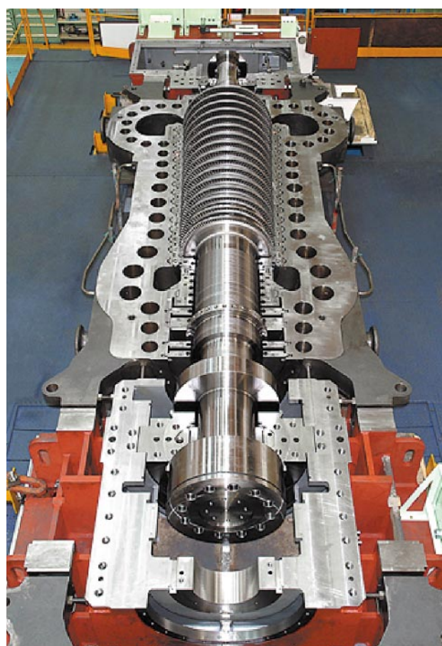
Fig. 8—External View of the High-pressure Turbine Rotor in the Steam Turbine of a Combined-cycle Power Plant.
