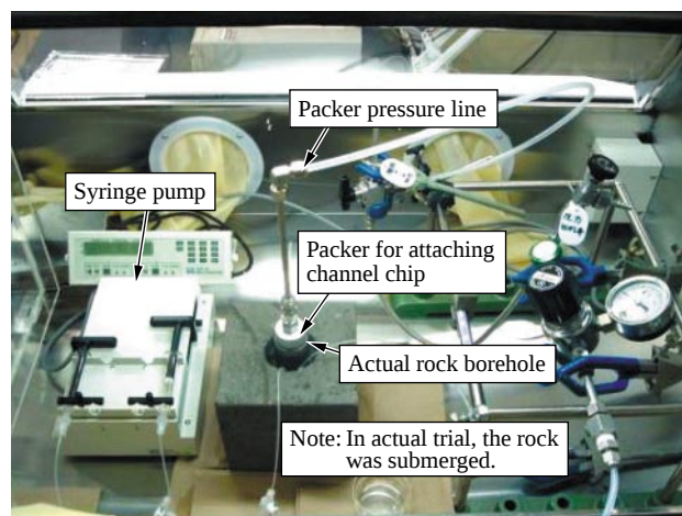
Fig. 3—Borehole Radionuclide Permeation Test Setup. Radionuclide migration tests were performed in an actual hole bored into a block of granite.
