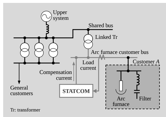
Fig. 7—Power System Circuit Configuration.
