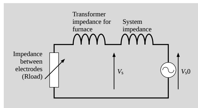
Fig. 6—Arc Furnace Equivalent Circuit.
