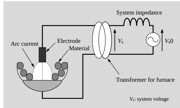
Fig. 5—Arc Furnace Schematic.
